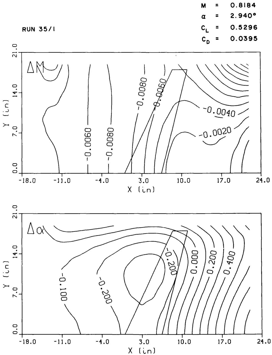
FIG. 10: MACH NUMBER AND ANGLE OF ATTACK CORRECTIONS, WING "A", M = 0.82 , \alpha = 2.94^\circ
