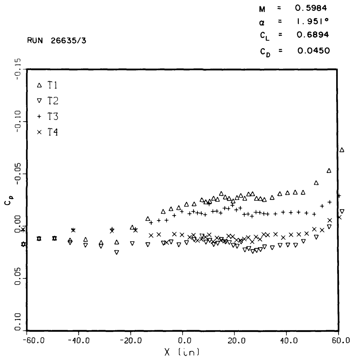
FIG. 5: TUBE PRESSURE DISTRIBUTIONS, M = 0.60 , \alpha = 1.95^\circ
