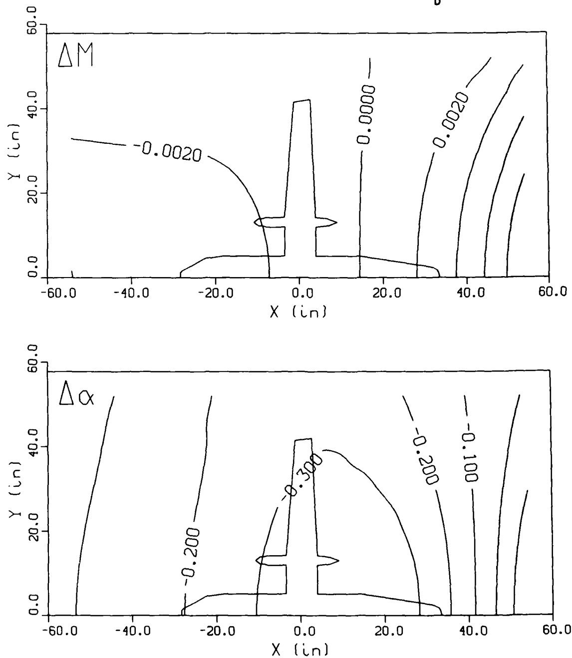
FIG. 7: MACH NUMBER AND ANGLE OF ATTACK CORRECTIONS, M = 0.60, \alpha = 1.95^\circ (200 PANELS)
