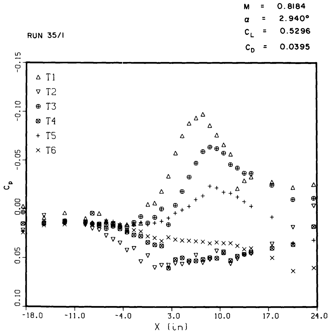
FIG. 9: RAIL PRESSURE DISTRIBUTIONS, WING "A", M = 0.82 , \alpha = 2.94^\circ
