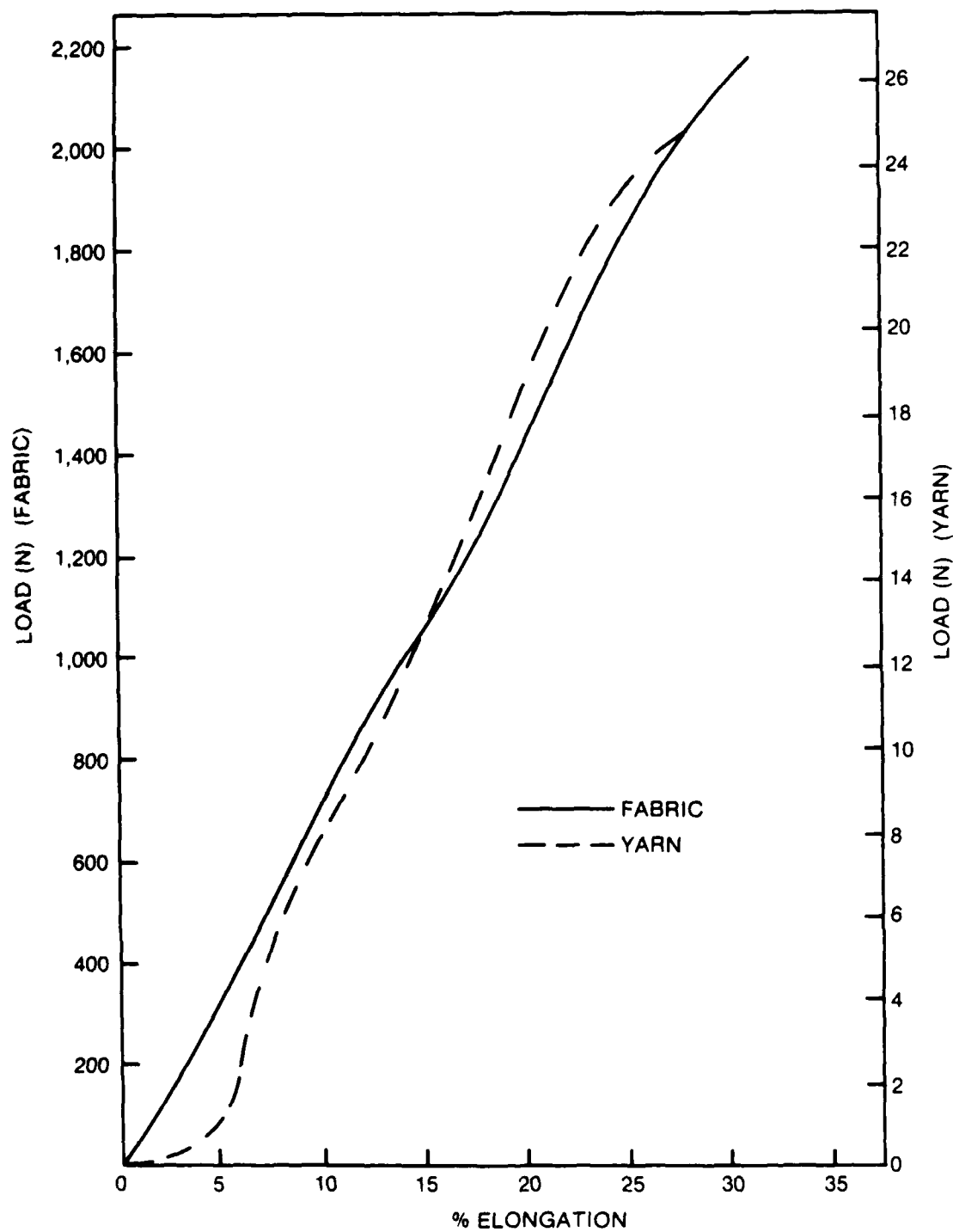
Figure A-3: The Load-Elongation Curves of Nylon Wary at -40^{\circ}\text{C} .
