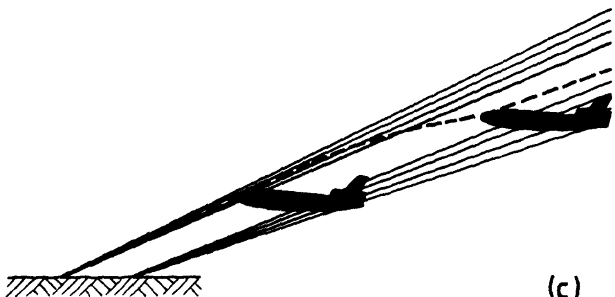
FIG. A2 THREE METHODS OF APPROACH WITH 2-BAR PAPI (not to scale)
