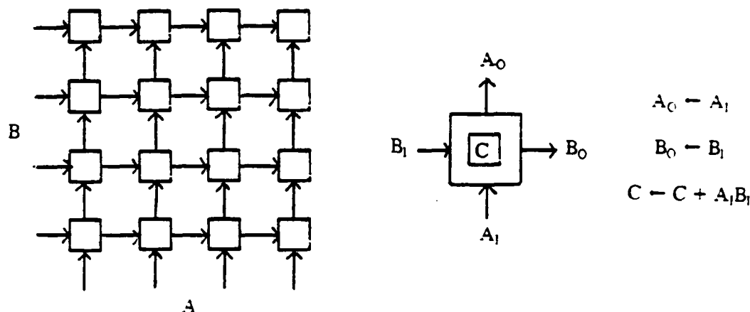
Figure 11. General structure of the canonical (I \ 0)^T matrix multiplier and functional description of modules
