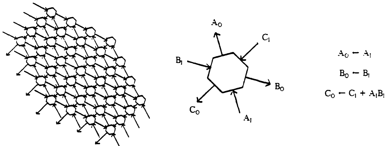
Figure 14. General structure of the [-1/3 \ -1/3]^F matrix multiplier
