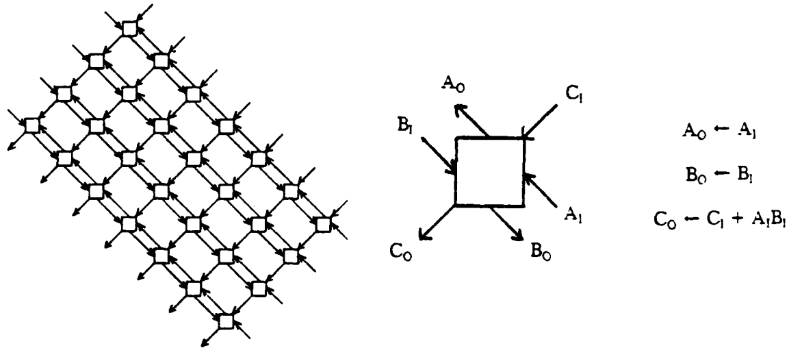
Figure 13. General structure of the [-1/2 \ -1/2]^F matrix multiplier
