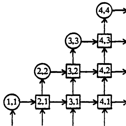
Figure 29. A [0 \ -1]^F network for triangular system solution
