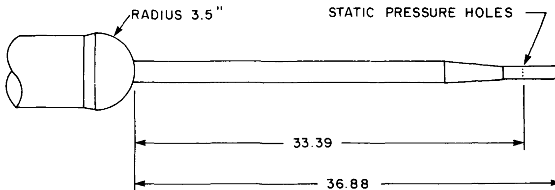
FIG. 3: SCHEMATIC AND DIMENSIONS OF THE PROBE IN THE SHORT AND EXTENDED CONFIGURATIONS
