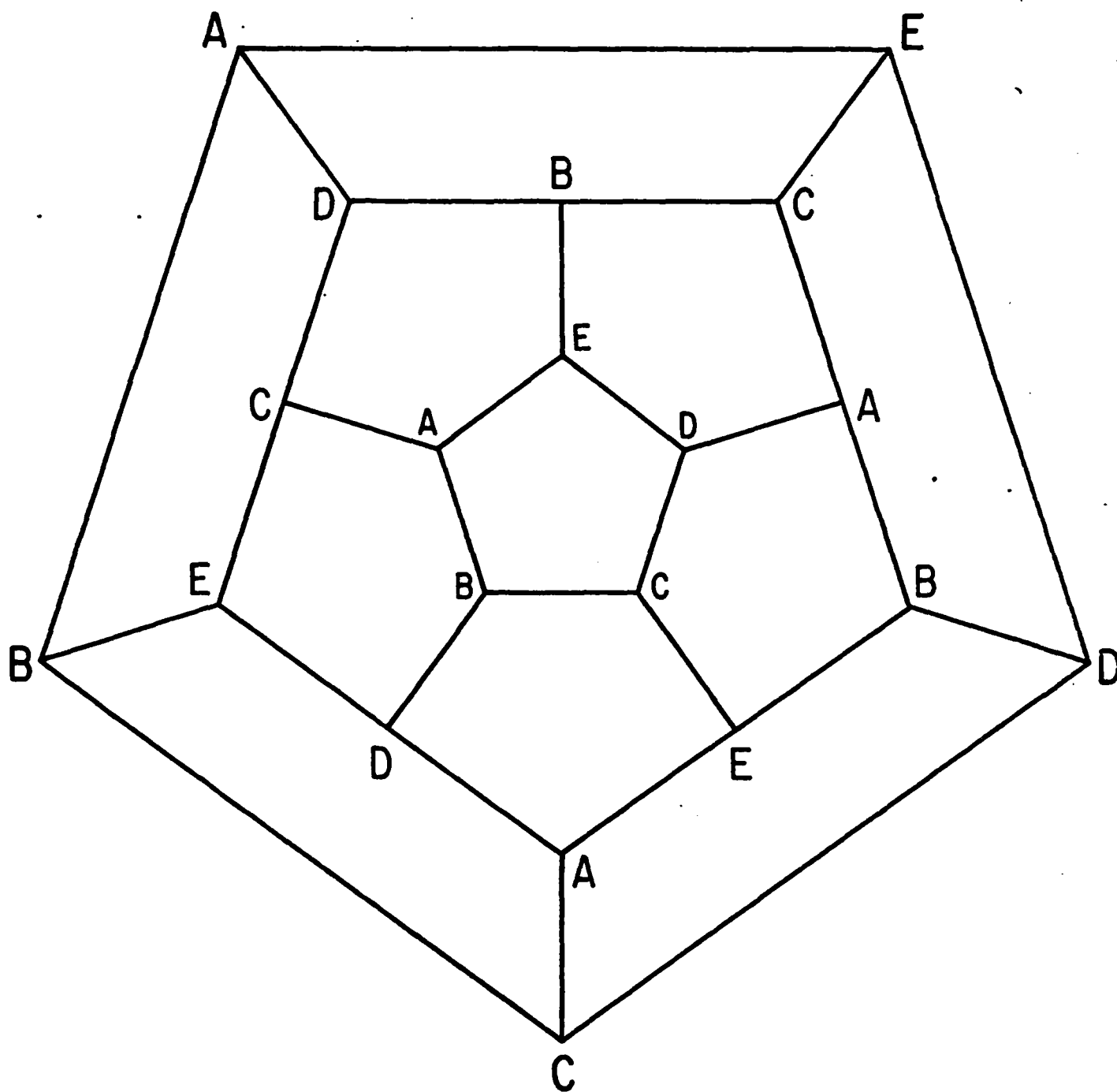
Figure 2. The relative positions of the five sets of four vertices on a regular dodecahedron.
