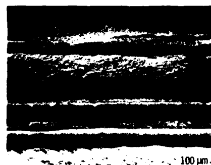
Figure 7. - Fracture surface of a 23 vol% SiC/RBSN composite tested in transverse flexure showing interfacial splitting between fiber and matrix.
