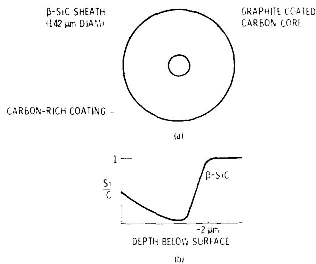
Figure 1. (a) Schematic of cross section of CVD SiC fiber. (b) The composition profile of carbon-rich coating on the surface of SiC fiber (AVCO SCS-6 fiber).
