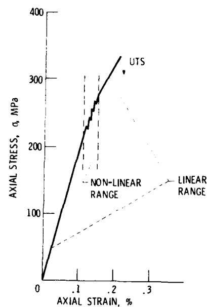
Figure 5. - The tensile stress-strain behavior for 20 vol% SiC fiber/RBSN composite showing linear and non-linear ranges.
