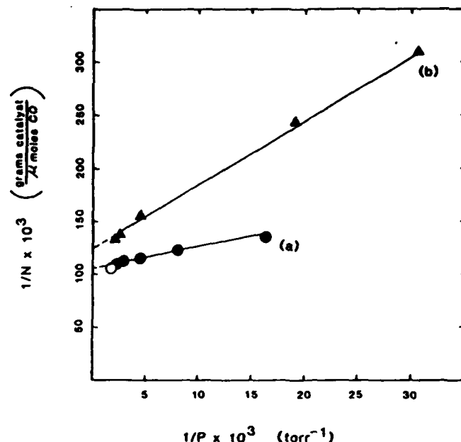
FIG. 5. Langmuir plots for CO chemisorption at 125°C: (a) (●) on Ni/Ti 2 O 3 (LT) and (b) (▲) on Ni/Ti 2 O 3 (HT). (The open symbol (○) corresponds to the uptake measurement influenced by the formation of Ni(CO) 4 .)
