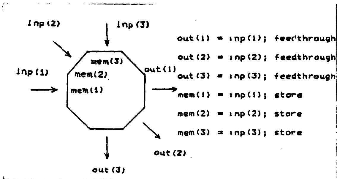
Figure 3.3 Buffer Cell
