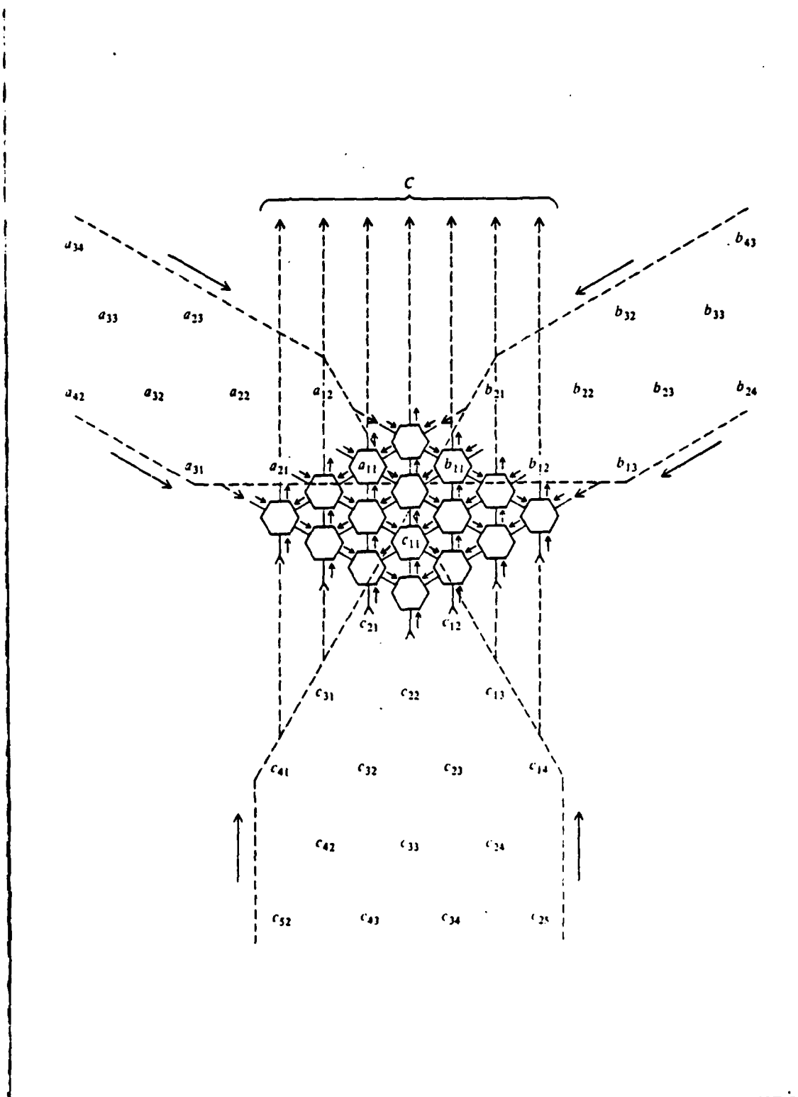
Figure 4.7 Systolic Array for Matrix-Matrix Multiplication
