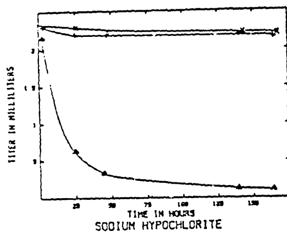
FIGURE I: Graphical presentation of data from chlorine-based oxidants. X is cold temperature, + is ambient, Δ is hot.
