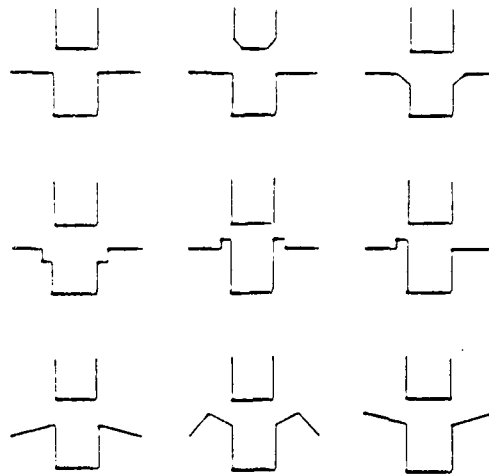
Figure 2. Similar peg-in-hole tasks that require different strategies.
