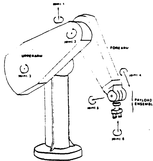
Figure 9. Unimation PUMA manipulator.
