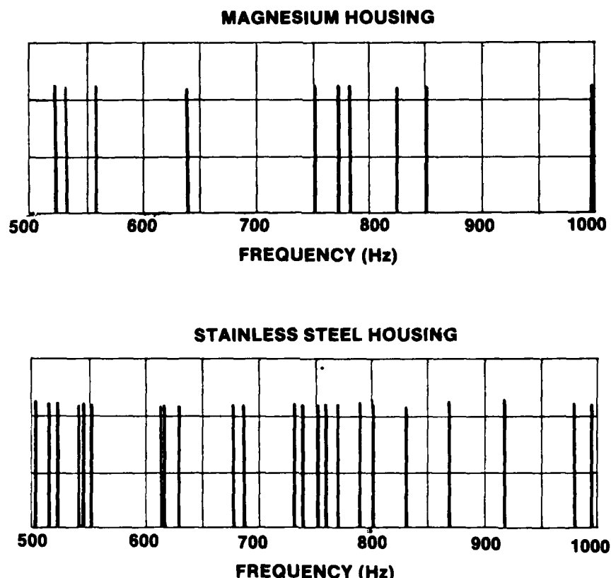
Figure 60. NASTRAN Calculated Natural Frequencies.
