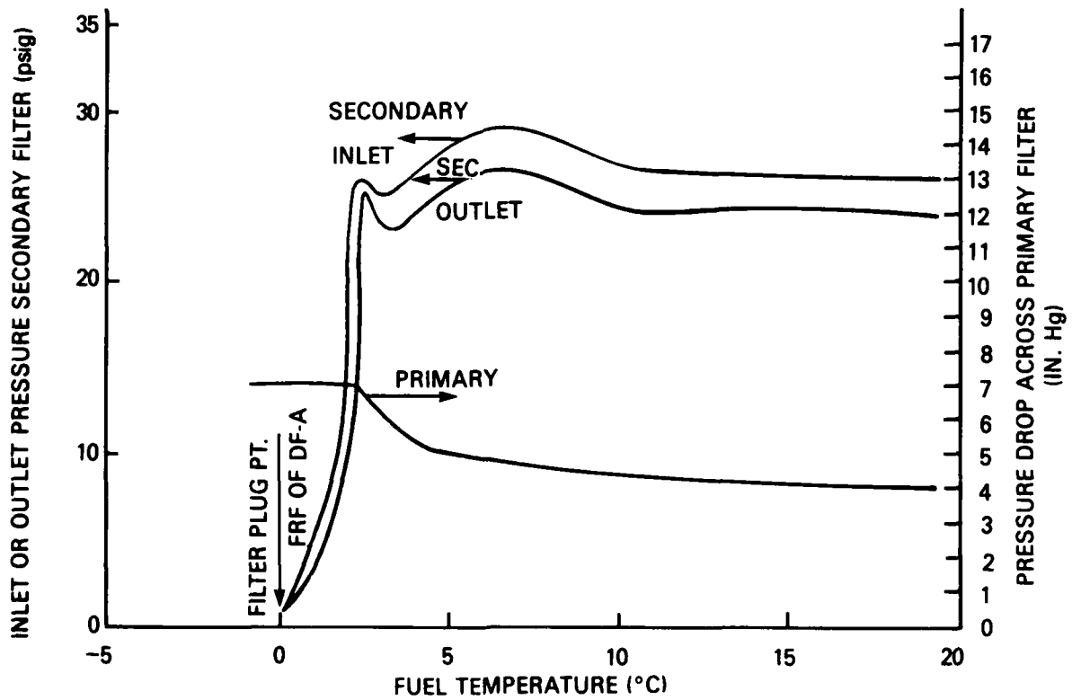
FIGURE 10. FRF OF DF-A - LOW-TEMPERATURE FILTERABILITY IN SIMULATED DD 6V-53T FUEL SYSTEM
