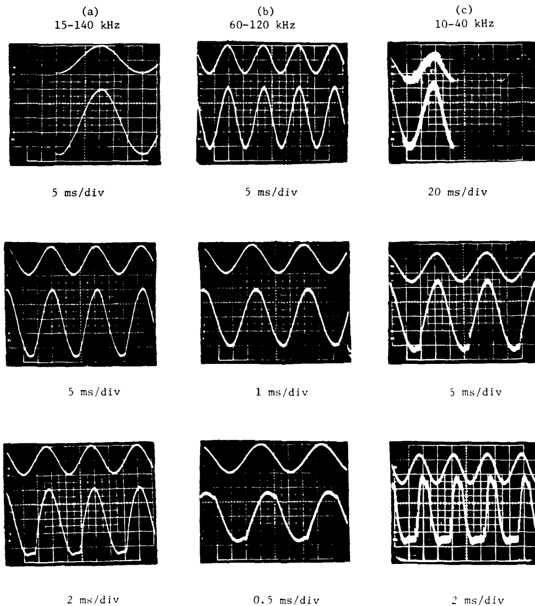
FIGURE 17 - Results of the agility tests to which the tracking filter was subjected. At (a), a sinusoidal frequency sweep from 15 to 140 kHz is applied at 35, 60 and 150 Hz respectively; at (b), a sinusoidal frequency sweep from 60 to 120 kHz is applied at 75, 275 and 450 Hz; at (c) a sinusoidal frequency sweep from 10 to 40 kHz is applied at 16, 55 and 200 Hz. In each case, the upper trace represents the modulation of the frequency generator while the lower trace is the actual voltage at the output of the F/V converter.
