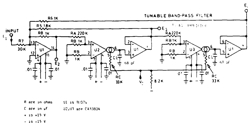
FIGURE 9 - Model of a second-order band-pass filter using operational transconductance amplifiers
