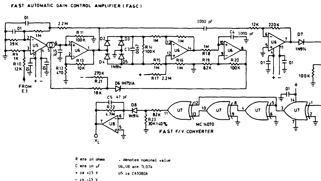
FIGURE 14 - Automatic gain control amplifier and frequency-to-voltage converter
