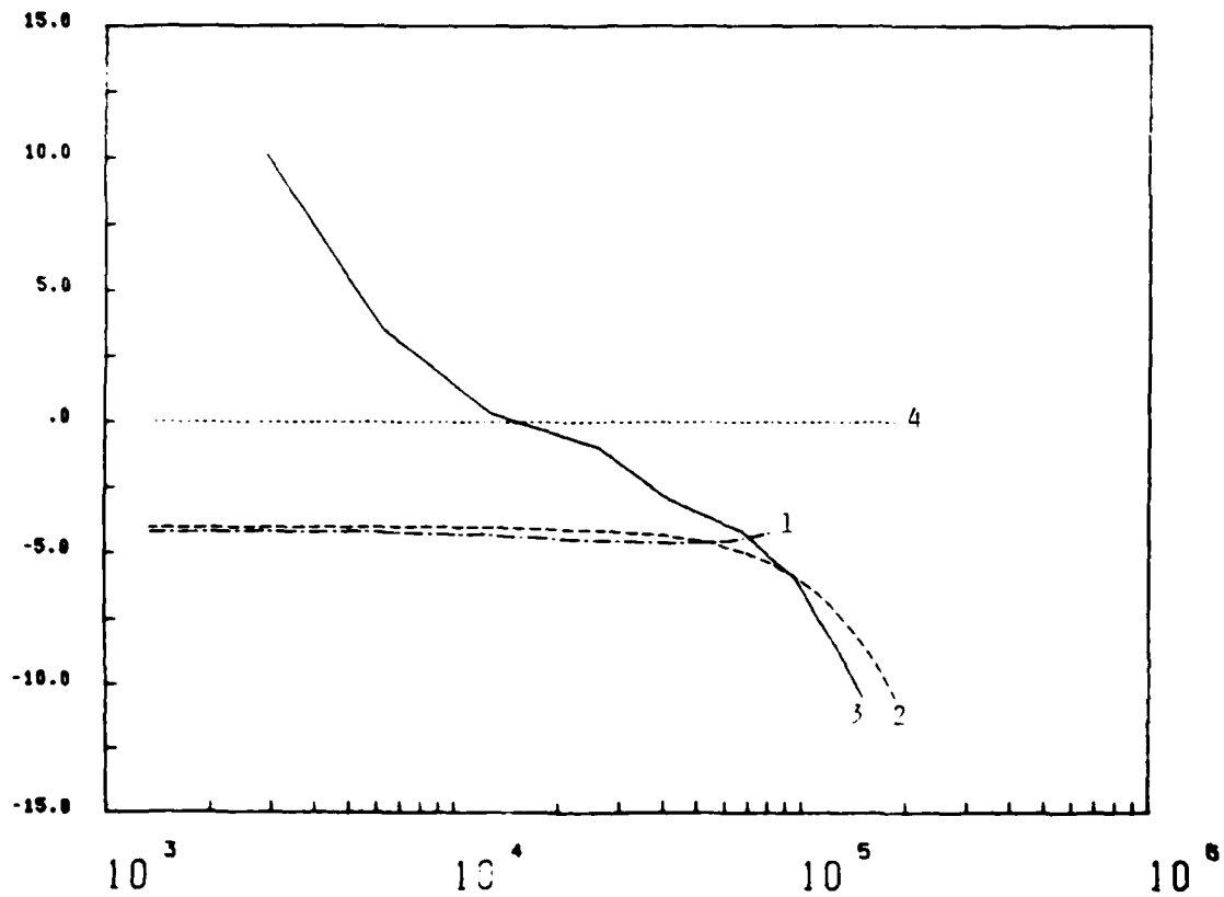
FIGURE 7 - Relative error of the control voltage as a function of the resonant frequency f_0
