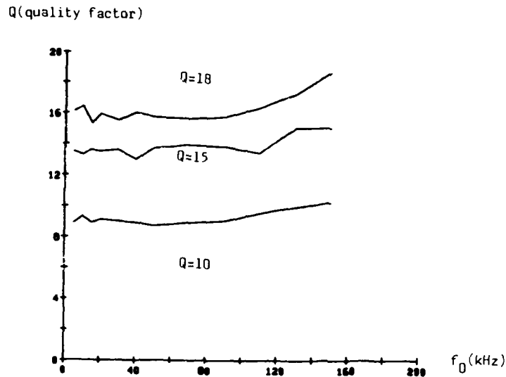
FIGURE 10 - Behavior of the quality factor of the band-pass filter built with OTAs as a function of the resonant frequency for various values of Q
