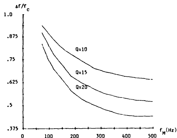
FIGURE 2 - Maximum values of the ratio \Delta f/f_c (frequency deviation to carrier frequency) as functions of the frequency of the modulating input signal for three values of the quality factor Q (10, 15 and 20). The frequency-tracking loop of the processor has a time constant of 650 \mu s while the AGC amplifier has a time constant of 1 ms and an amplitude dynamic range of 60 dB.
