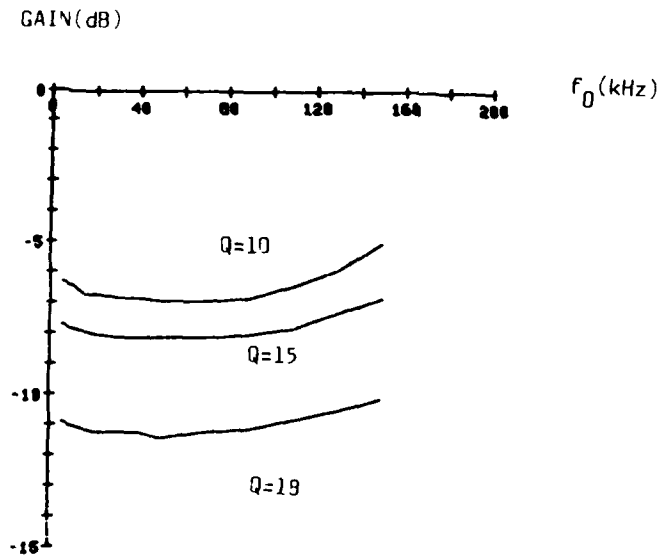
FIGURE 11 - Behavior of the gain of the filter built with OTAs as a function of the resonant frequency when the factor of quality is set to 10, 15 and 18.
