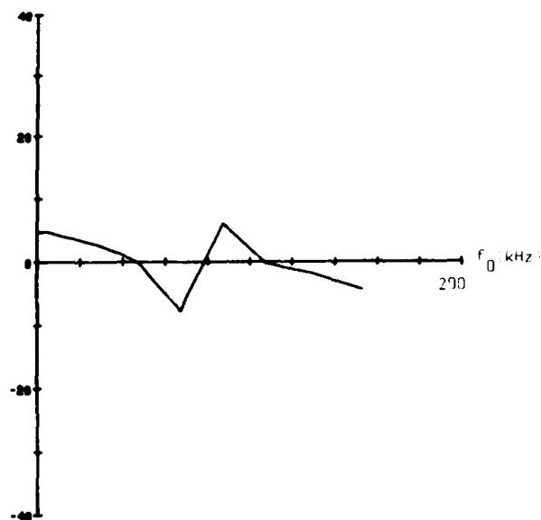
FIGURE 12 - Relative error of the resonant frequency control voltage of the band-pass filter built with OTAs as a function of the resonant frequency
