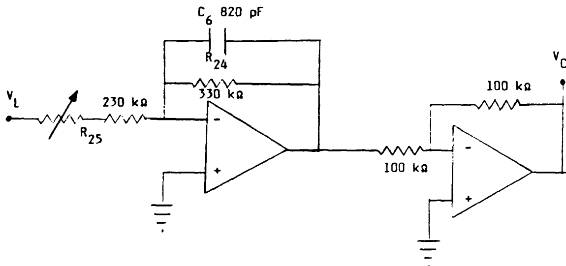
a) for band-pass filter built with multipliers
