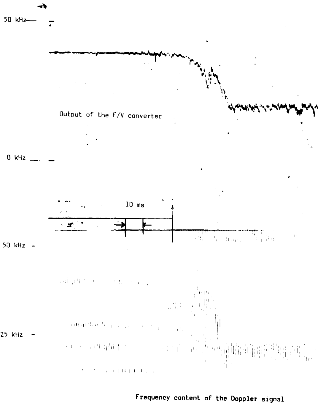
FIGURE 20 - Response of the frequency-tracking filter to a Doppler signal characterized by strong interference
