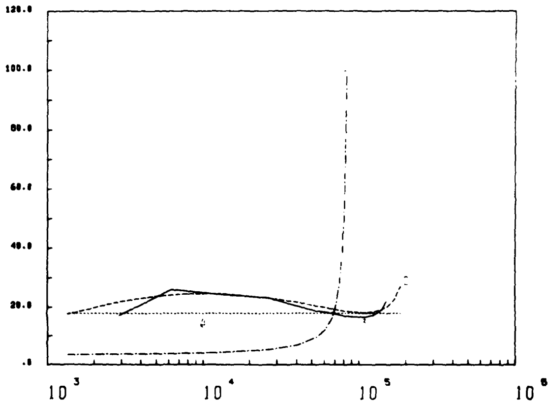
FIGURE 4 - Behavior of the quality factor of the band-pass filter as a function of the resonant frequency f_0
