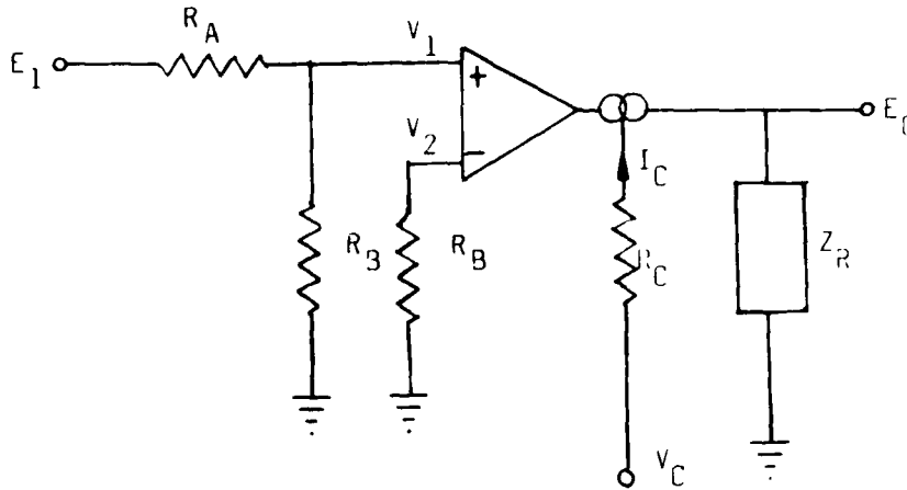
FIGURE 8 - Operational transconductance amplifier as a variable transfer function
