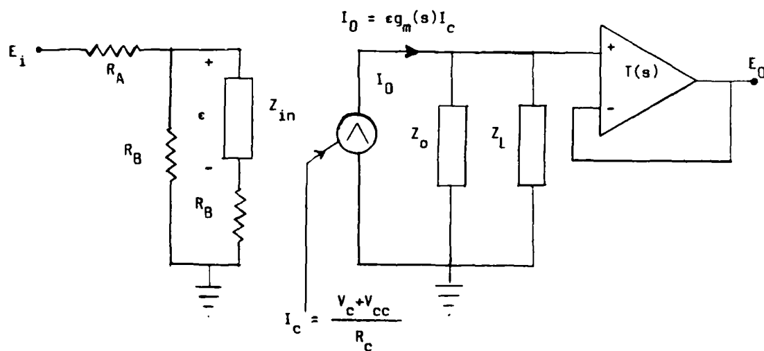
FIGURE 13 - Model of a nonideal operational transconductance amplifier
