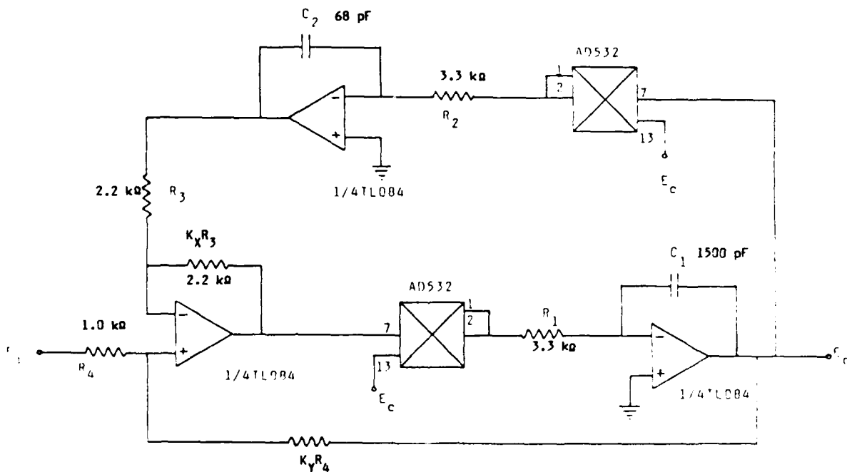
FIGURE 3 - Second-order tunable band-pass filter realized by two multipliers
