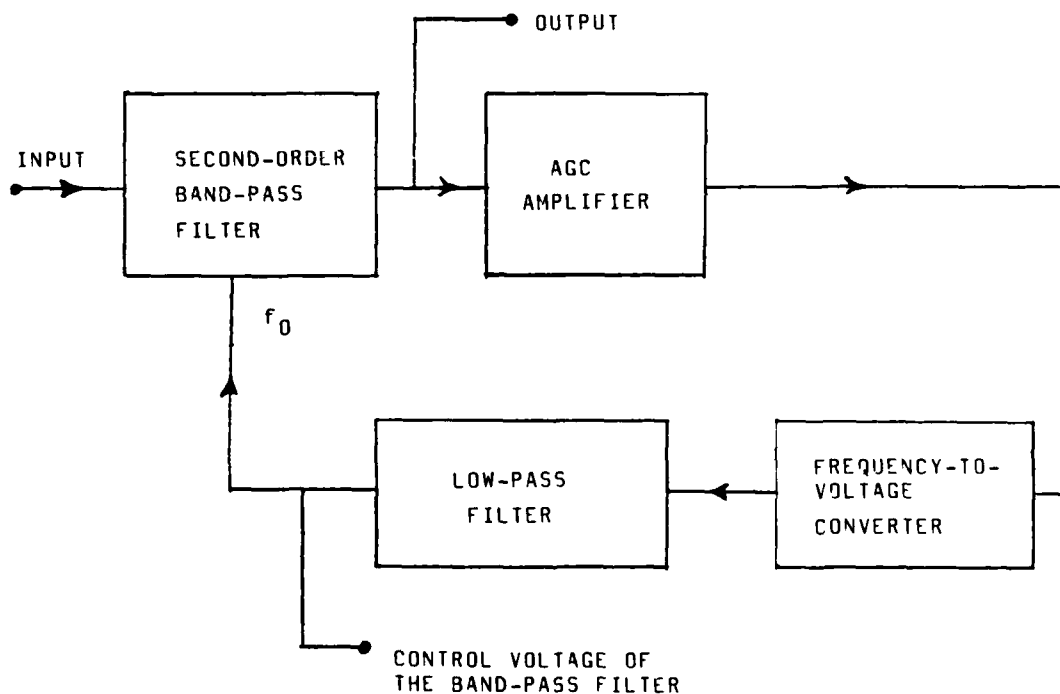
FIGURE 1 - Schematic of the frequency-tracking filter
