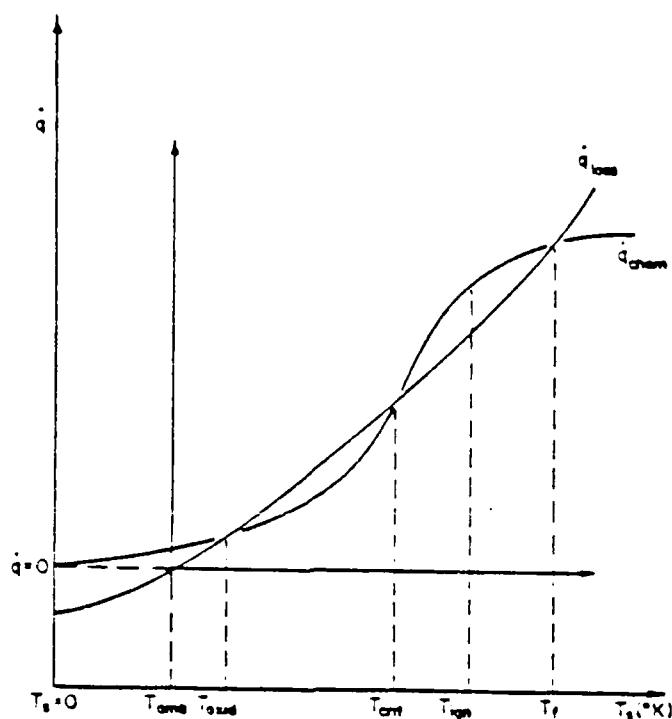
Figure 4.3. Summary Plot of \dot{q} versus T_s . Taken from [Ref. 28]
