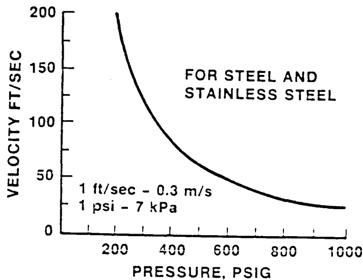
Figure 3.17. CGA Curve of Vel/Pressure Taken from [Ref. 18]
