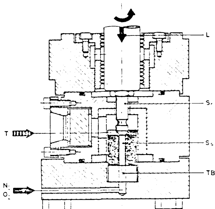
Figure 3.11. Schematic of Jenny and Wyssmann's Test Apparatus for Ignition Tests. L = Axial Load, S_r = Rotating Specimen, S_s = Stationary Specimen, T_B = Torque Strain Gage Balance, and T = Temperature Measurement with Pyrometer. Taken from [Ref. 14]
