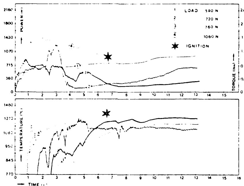
Figure 3.12. Temperature and Friction Power Records From Oxygen Tests ( O_2 ) with GGG 40 ( S_x ) and X20Cr13 ( S_r )
