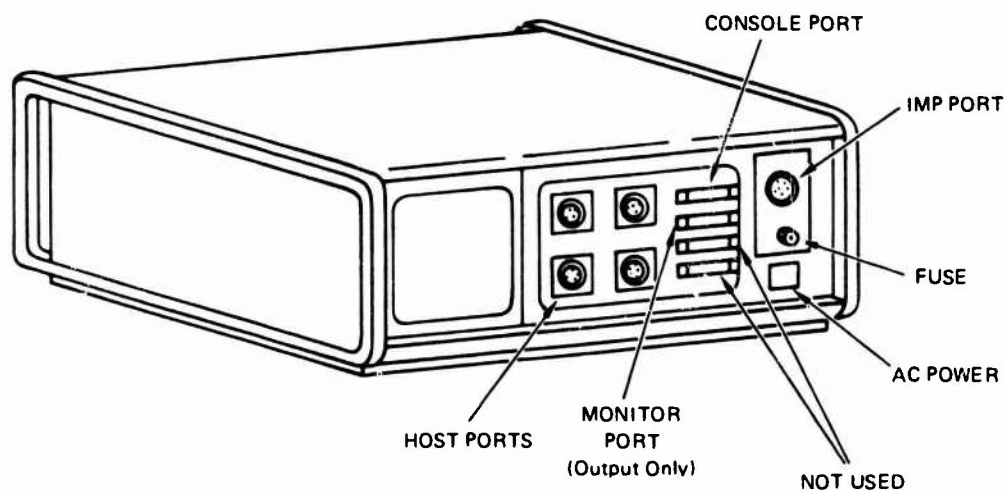
FIGURE 4 RUGGEDIZED CONFIGURATION
