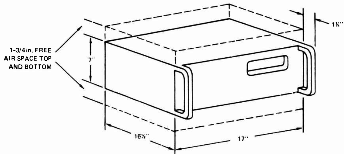
RUGGEDIZED CONFIGURATION
