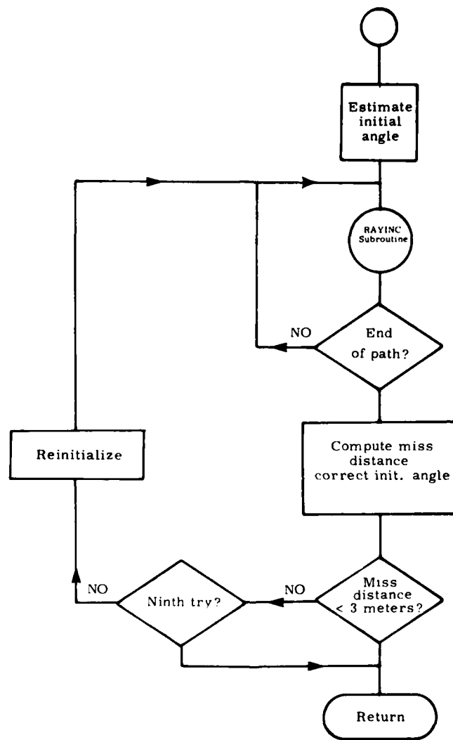
Figure 5c. SEARCH Subroutine
