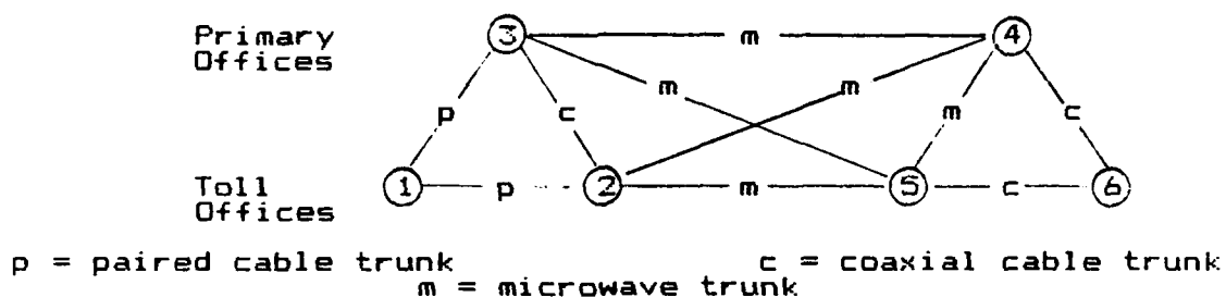
Figure 6.23 Class 3 and 4 Structure with Various Media
