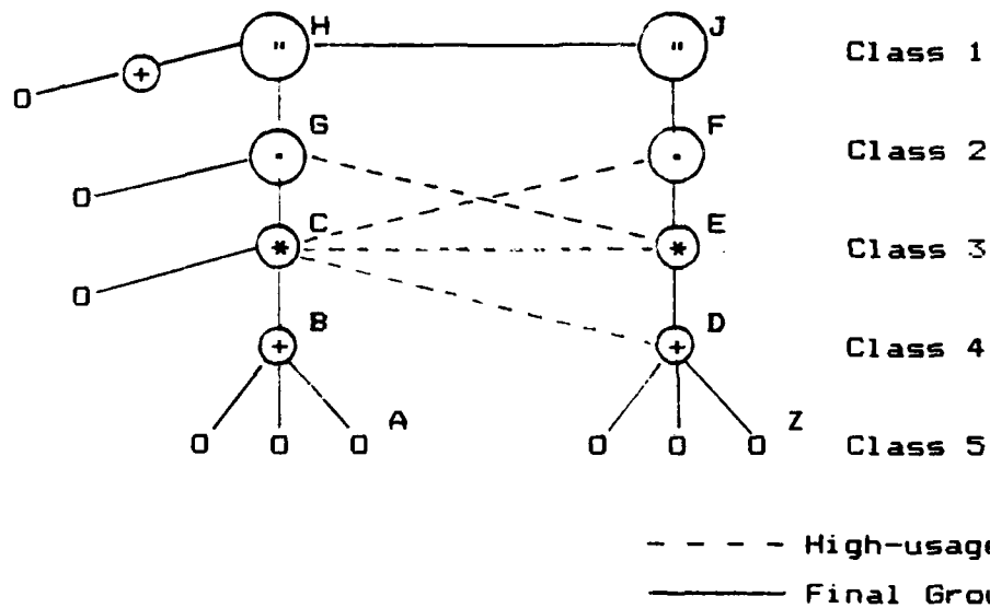
Figure 3.5 Nominal Toll Network Switch Pattern
