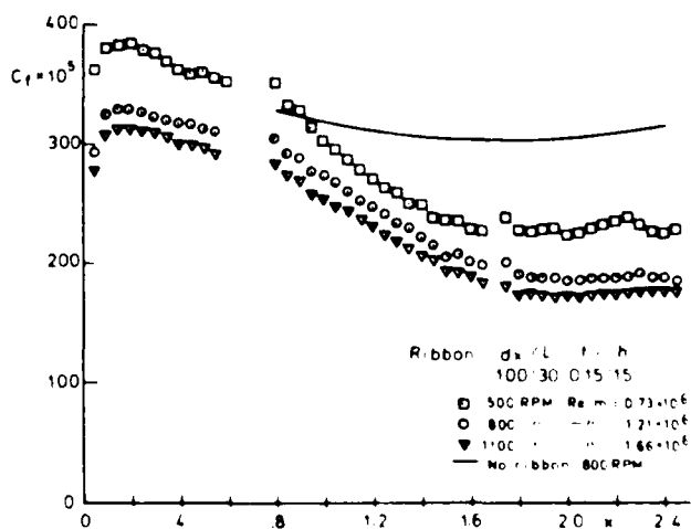
Figure 1. Local skin friction as function of position ( dx/L = 2.33 , t/h = 0.15 ) (from Bertelrud, Truesd, and Avellan, 1982; reproduced by permission of the American Institute of Aeronautics and Astronautics, Inc.).
