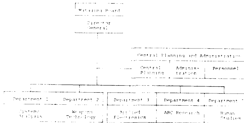
Figure 2. FOA organization.
