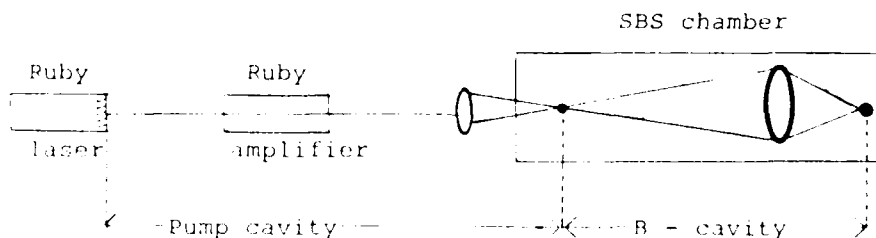
Figure 3. Phase-conjugate resonator.
