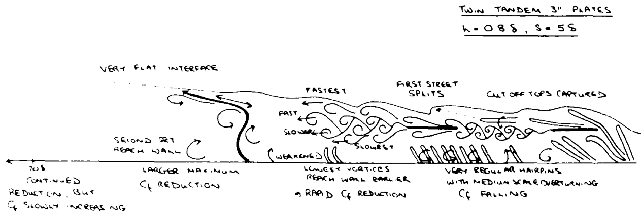
Figure 3. Operation of tandem LEBU in outer portion of turbulent boundary layer (Mumford and Saville, 1983; reproduced by permission of the American Society of Mechanical Engineers).
