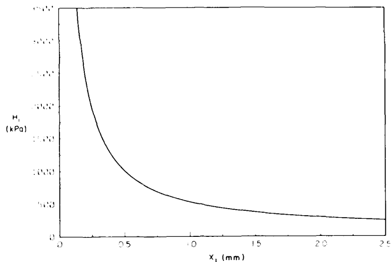
Figure 14. Hardness value H_i versus the hardness index x_i according to eq 10.
