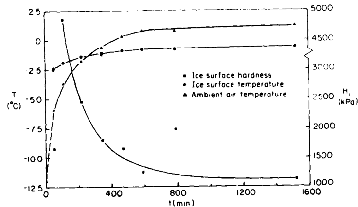
Figure C1. Hardness H , and temperature T history of ice during warmup.
