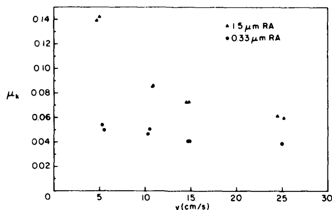
Figure 24. Effect of roughness R and velocity v on the kinetic friction coefficient \mu_k between stainless steel samples and ice ( P = 10 \text{ kPa} , H_i = 2800 \text{ kPa} ).
