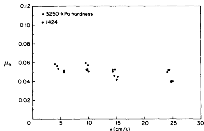
Figure 27. Effect of ice hardness H_i and velocity v on the kinetic friction factor \mu_k between a sample of stainless steel (0.33 \mu\text{m} RA) and ice ( P = 10 kPa).
