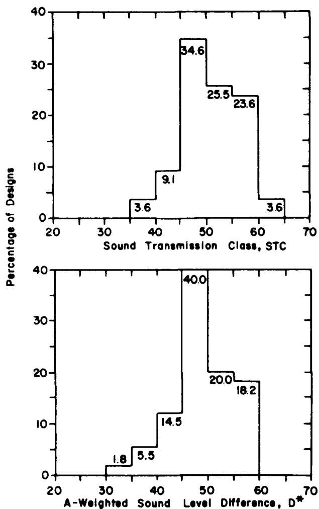
Figure 4.—Distributions of designs with STC and D* for wood-joist floor-ceiling assemblies contained in DuPree's (1981) data base. (ML84 5559)
