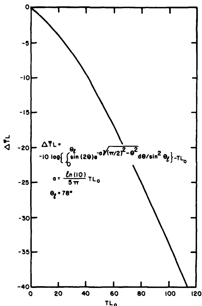
Figure C-2.—Plot of \Delta TL versus TL_0 for \theta_i = 78^\circ . (ML84 5564)
