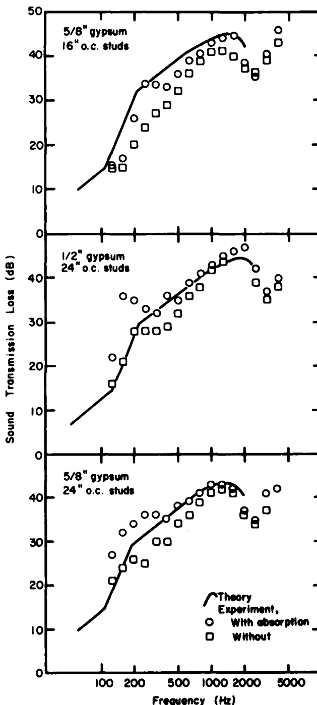
Figure D-1.—Comparison of theory and measurement for a single-row-of-stud wall with gypsum board attached directly to each side of a 2 x 4 wood-stud framework: Upper—5/8-inch-thick gypsum board on each side of studs 16 inches o.c. Central—1/2-inch-thick gypsum board on each side of studs 24 inches o.c. Lower—5/8-inch-thick gypsum board on each side of studs 24 inches o.c. (ML84 5565)
