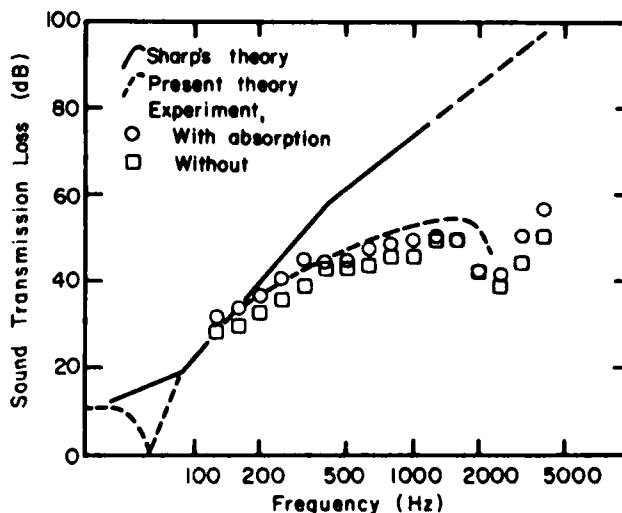
Figure 14.—Comparison of Sharp's theory, our theory, and measurement for a double-row staggered-stud wall with a single layer of 5/8-inch-thick gypsum board attached directly to 2 x 4 wood studs 16 inches o.c., staggered 8 inches o.c. on a 2 x 6 plate, with and without cavity sound absorption. (ML84 5555)
