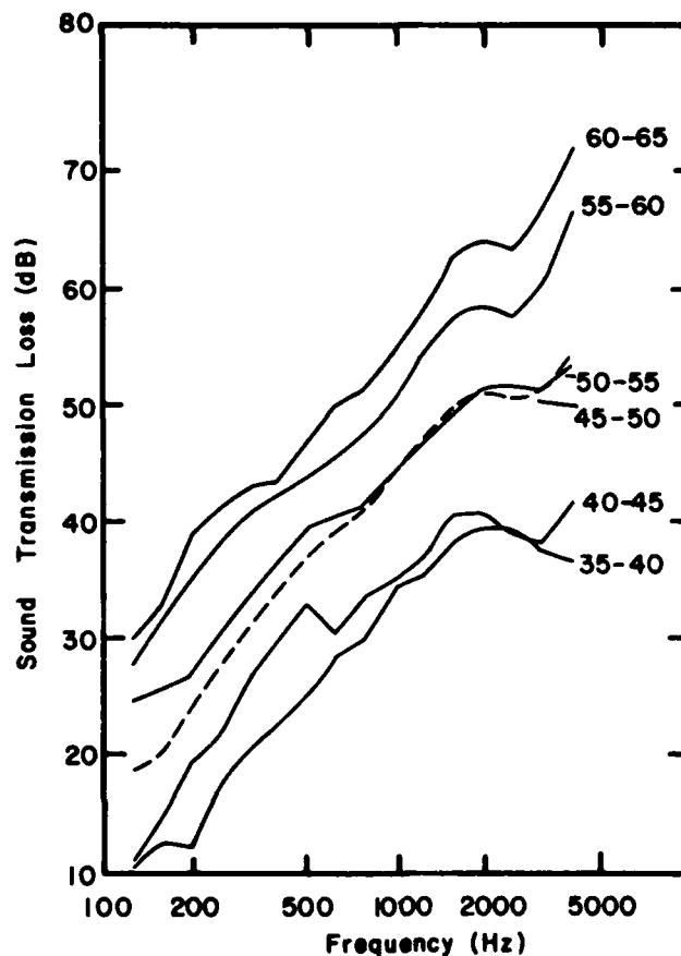
Figure 5.—Mean values of one-third-octave-band sound transmission loss for wood-joist floor-ceiling assemblies; data grouped by intervals of STC rating. (ML84 5560)
