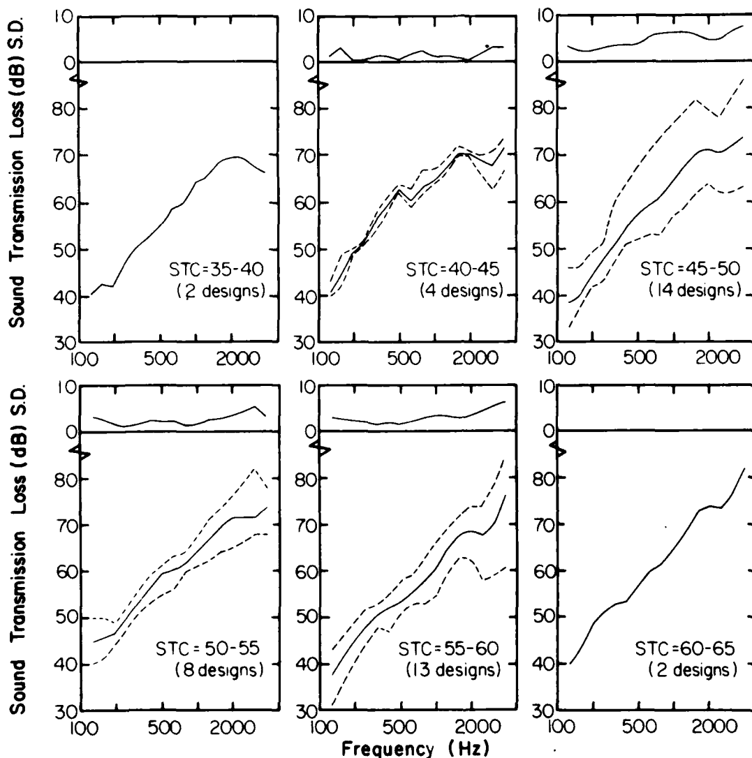
Figure A-3.—Mean value of one-third-octave-band sound transmission loss for wood-joint floor-ceiling assemblies for six STC rating intervals. (ML84 5573)
