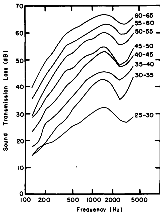
Figure 2.—Mean values of one-third-octave-band sound transmission loss for wood-frame interior partitions; data grouped by intervals of STC rating. (ML84 5558)
