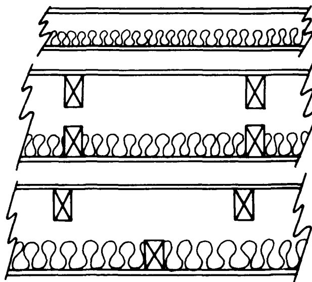
Figure 7.—Panel configurations for which prediction methods apply. ML84 5566)
