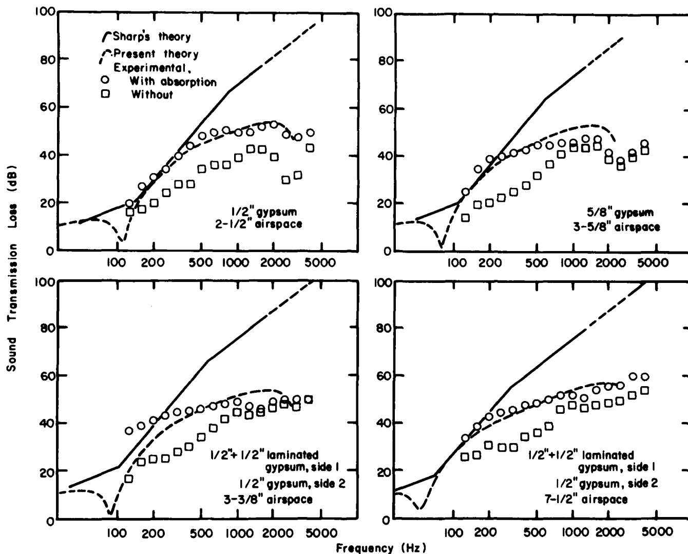
Figure D-2.—Comparison of theories and measurements for studless double-panel construction with gypsum board and airspace combinations with and without cavity sound absorption: Upper left—1/2-inch-thick gypsum board panels separated by a 2-1/2-inch airspace, Upper right—5/8-inch-thick gypsum board panels separated by a 3-5/8-inch airspace, Lower left—Two layers of 1/2-inch-thick gypsum board on one side of a 3-5/8-inch airspace, and one layer of 1/2-inch-thick gypsum board on the other, Lower right—Two layers of 1/2-inch-thick gypsum board on one side of 7-1/2-inch airspace, and one layer of 1/2-inch-thick gypsum board on the other. (ML84 5569)
