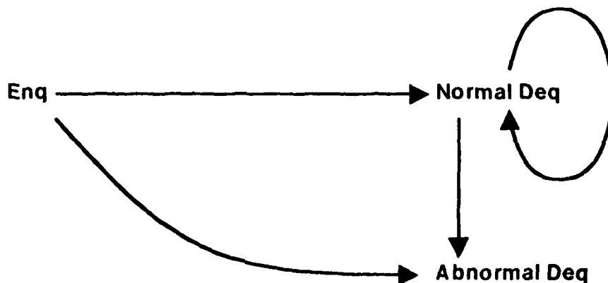
Figure 4a: The quorum intersection graph.
