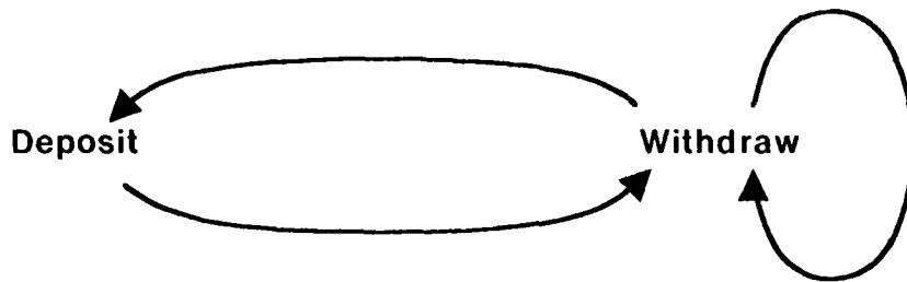
Figure 11a: The quorum intersection graph.
