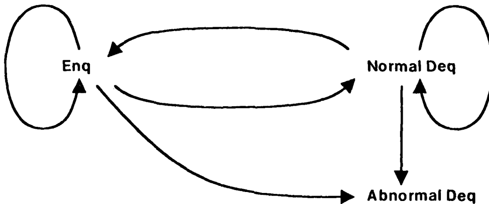
Figure 2a: The quorum intersection graph.
