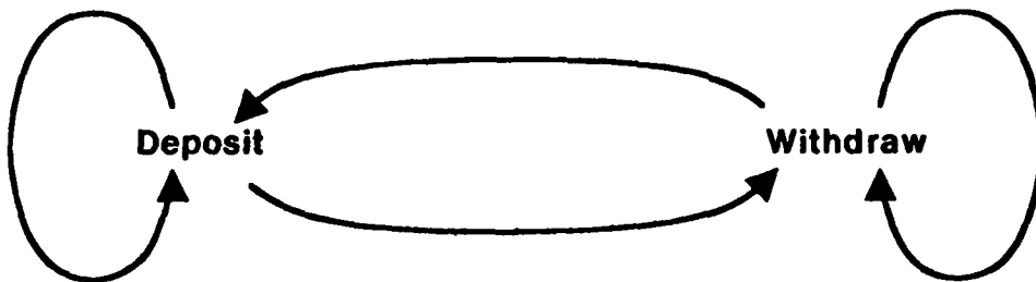
Figure 12a: The quorum intersection graph.
