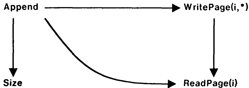
Figure 5a: Quorum Intersection Graph
