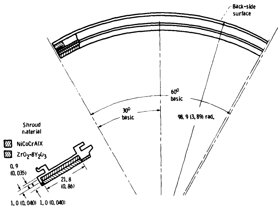
Figure 5. - Shroud general geometric parameters. (Dimensions are in millimeters (inches).)
