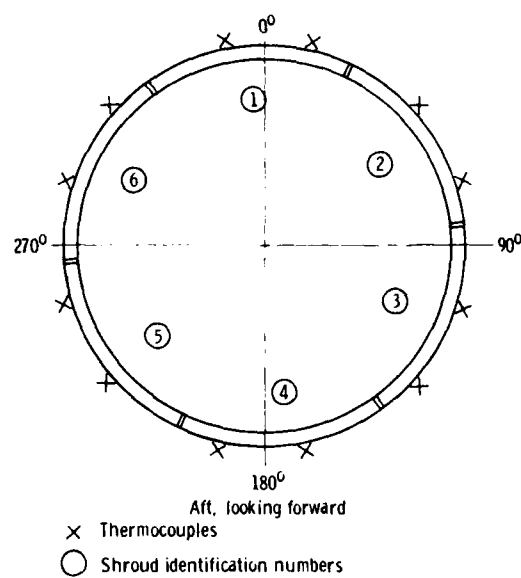
Figure 4. - Position of thermocouples on turbine tip shrouds.
