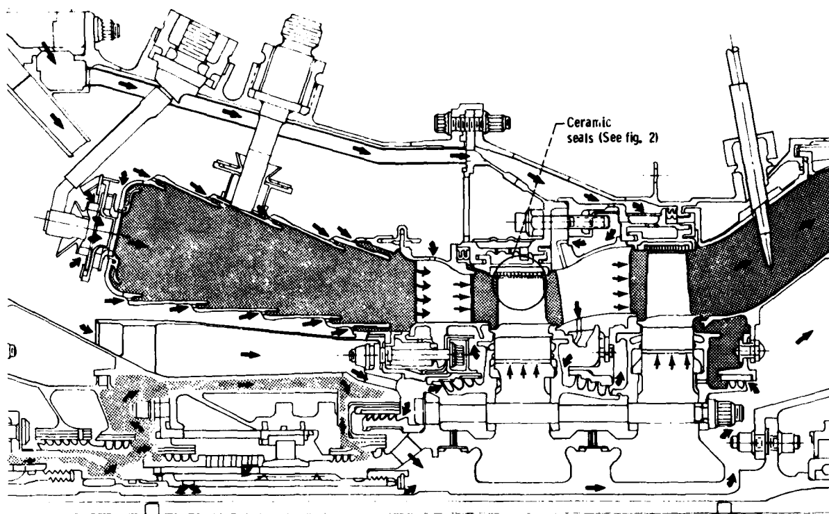
Figure 1. - Engine hot section schematic.
