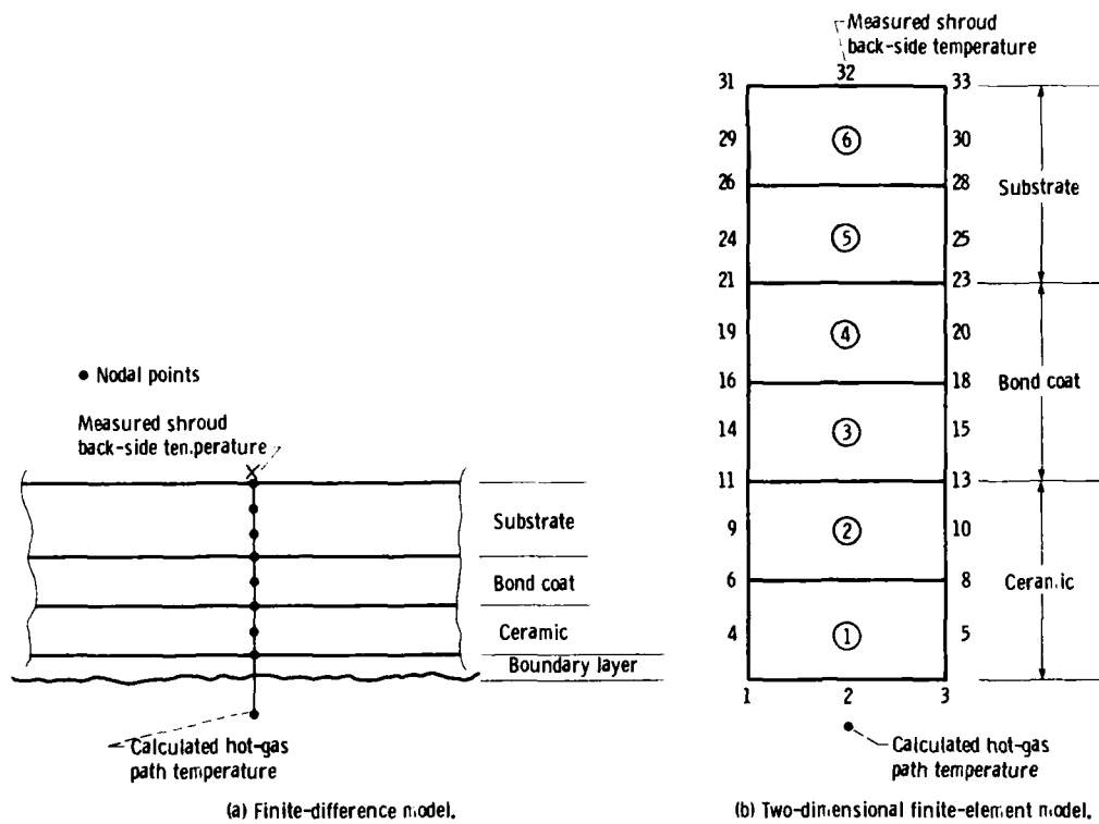
Figure 15. - Models used for heat-transfer calculations.
