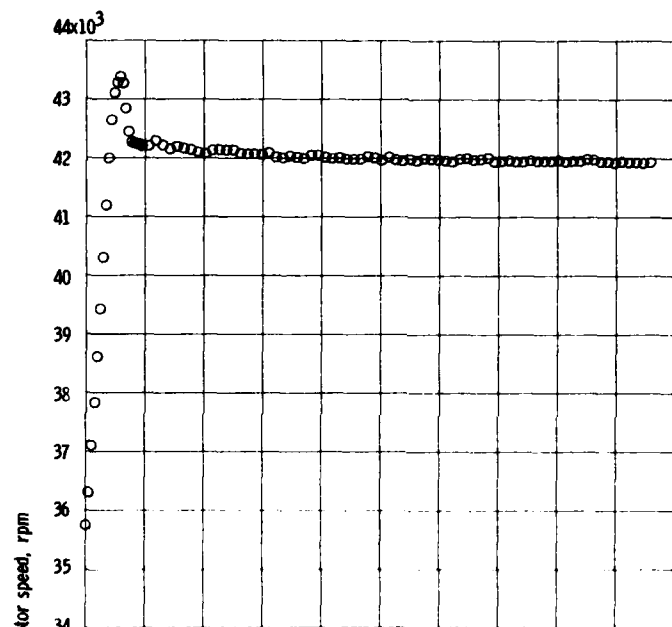
(a) Acceleration (heatup).
