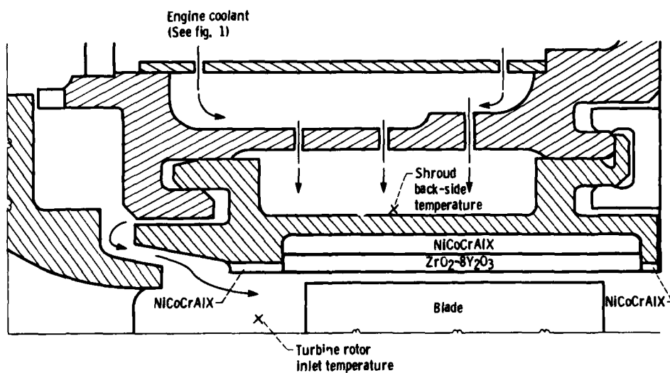
Figure 2. - Schematic of ceramic seal.
