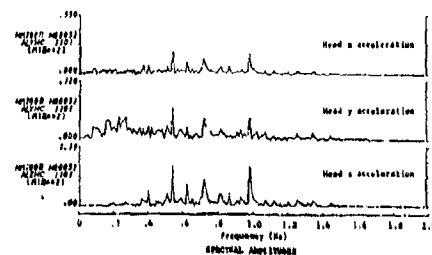
Figure 8b. Head x,y,z response of subject 32, seated, facing bow (nausea condition).
