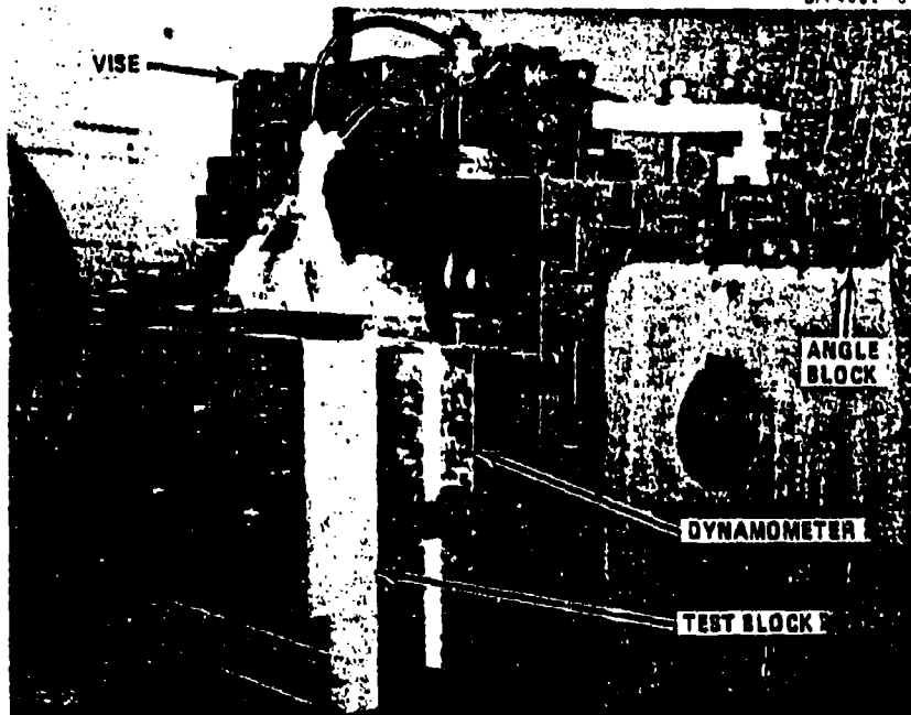
Figure 72. Three-Axis Milling Table Dynamometer and Test Setup
