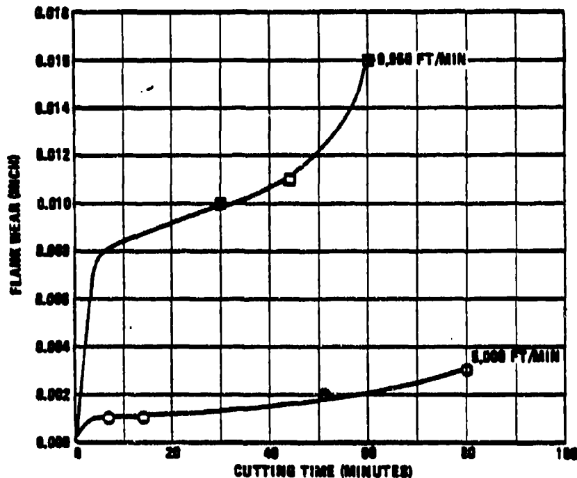
Figure 95. Approximate Effect of Cutting Speed on Cutter Wear
