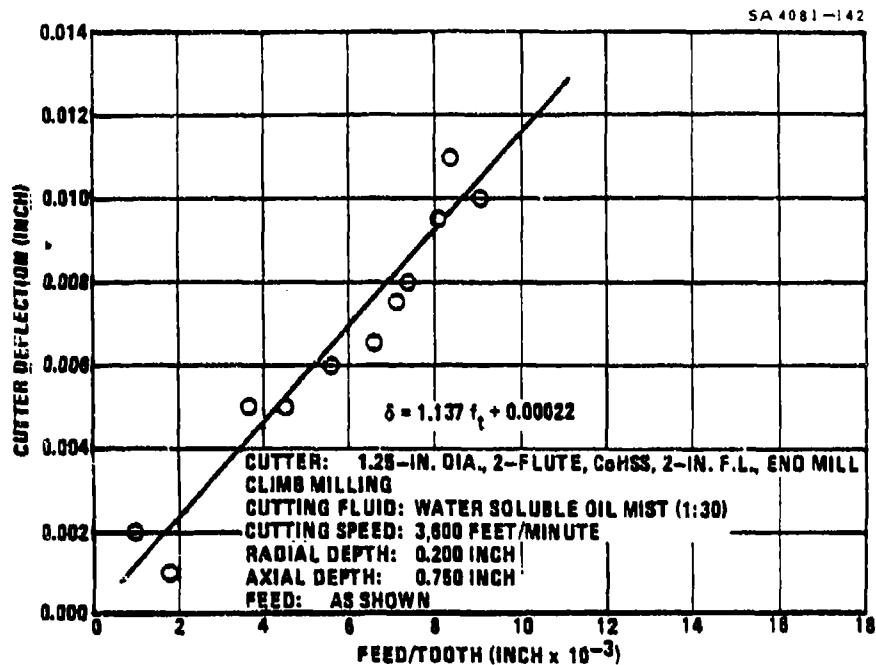
Figure 129. Effect of Feed Rate on Cutter Deflection for 6061-T651 Aluminum
