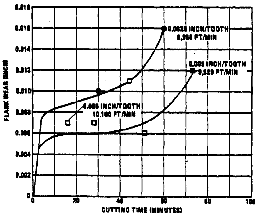
Figure 89. Effect of Feed Rates on Cutter Wear
