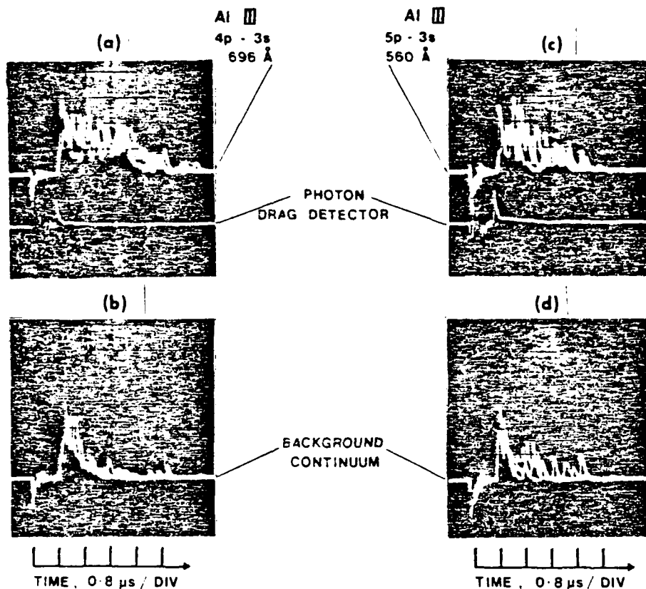
Fig. 13. Time-resolved AlIII line intensities in laser produced plasma: a) AlIII, 4p-3s, 696 Å intensity vs time; b) continuum background; c) AlIII, 5p-3s, 560 Å intensity vs time; d) continuum background. The lower trace in a and c is the signal from the photon drag detector which samples the Co 2 laser.
