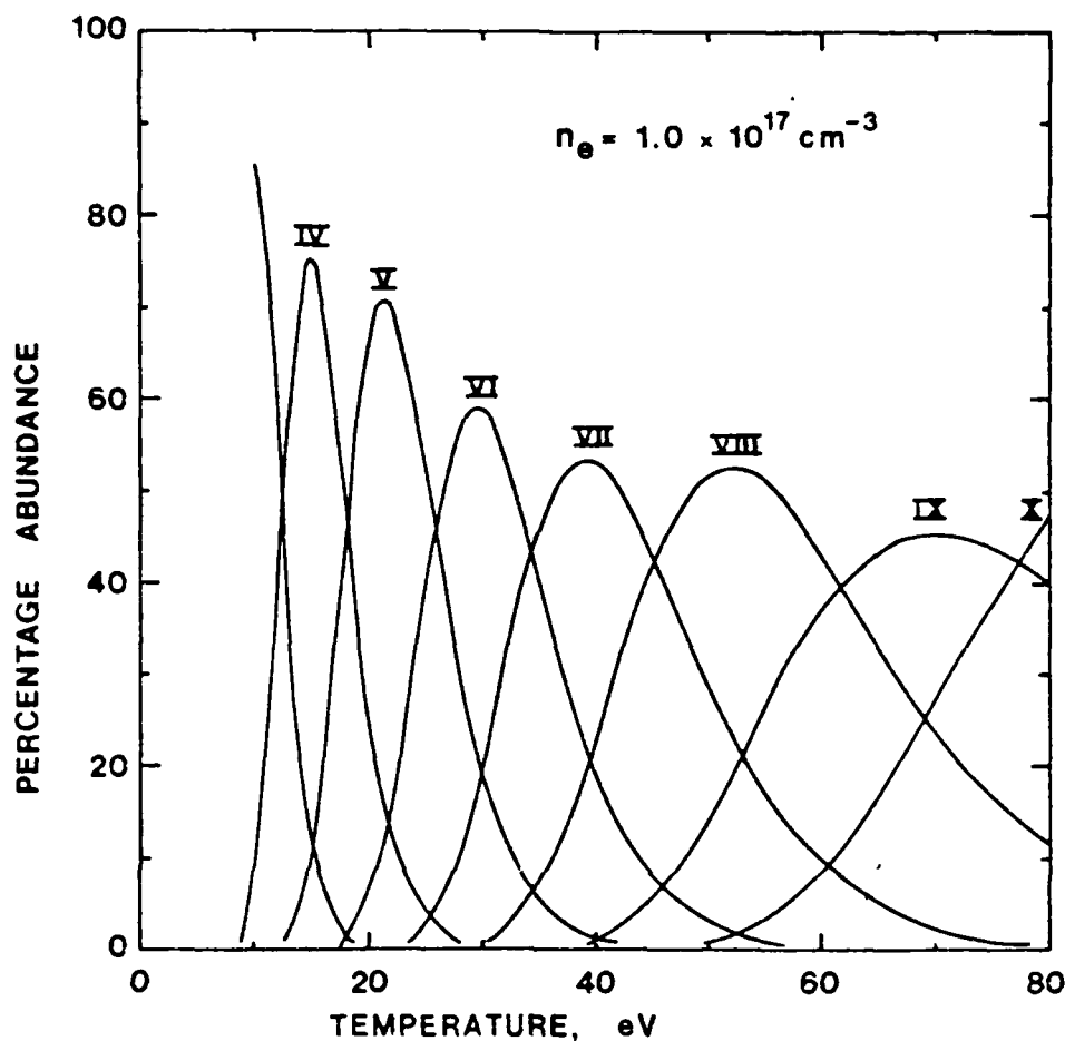
Fig. 5. Charge state distribution in a Sodium plasma, obtained from a modified coronal equilibrium model. The electron density is 10^{17} \text{ cm}^{-3} .
