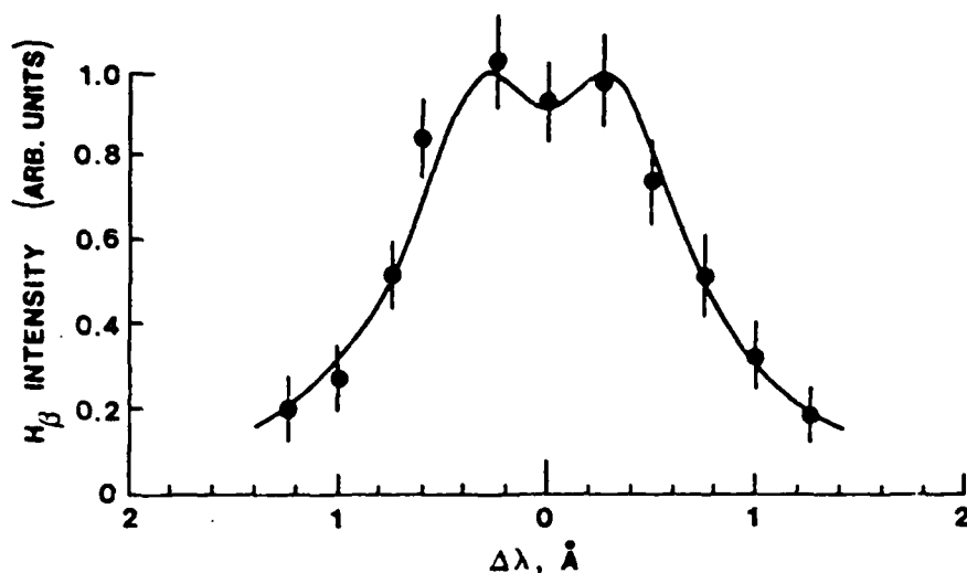
Fig. 9. H_\beta line intensity vs wavelength in the C discharge. The curve through the measured points is a convolution of a Stark profile with a Doppler profile.
