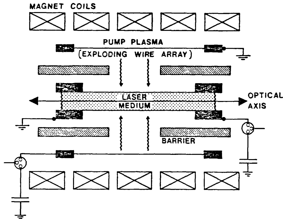
Fig. 2. Schematic diagram of proposed coaxial discharge arrangement.
