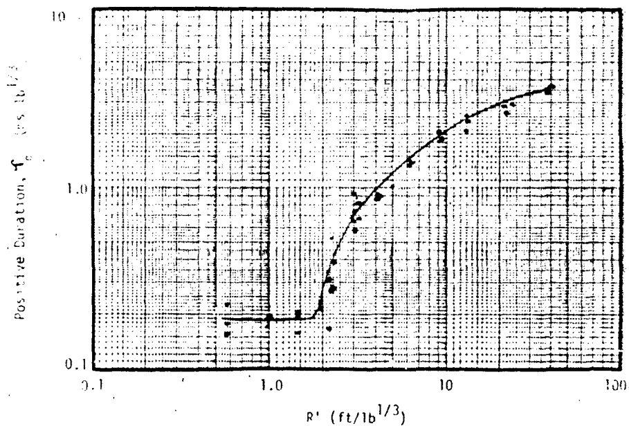
FIGURE 4-6. REDUCED POSITIVE PHASE DURATION ( \tau_p ) - DISTANCE FOR ANFO I, II, AND III. SCALED TO SEA LEVEL CONDITIONS.
