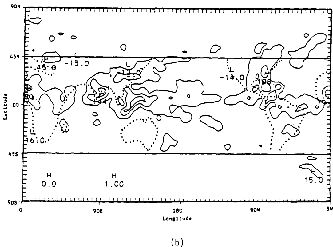
Figure 3.8. Precipitation and heating rates for 12 May - 18 May, 1979.
