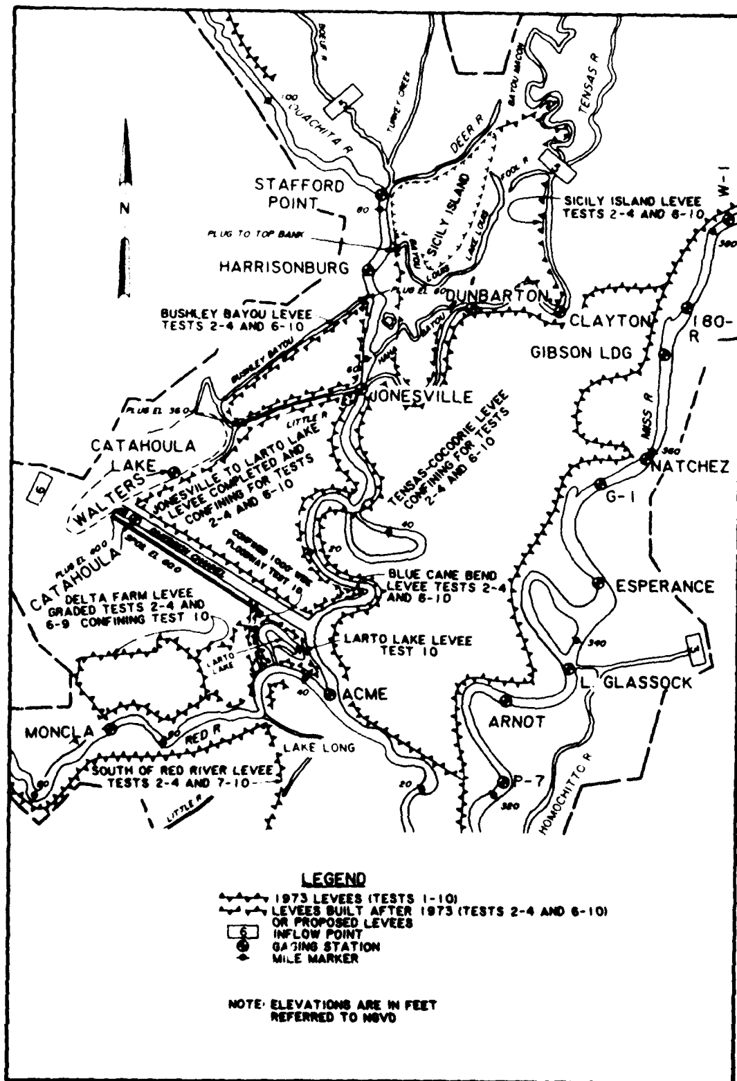
Figure 3. Levee conditions
