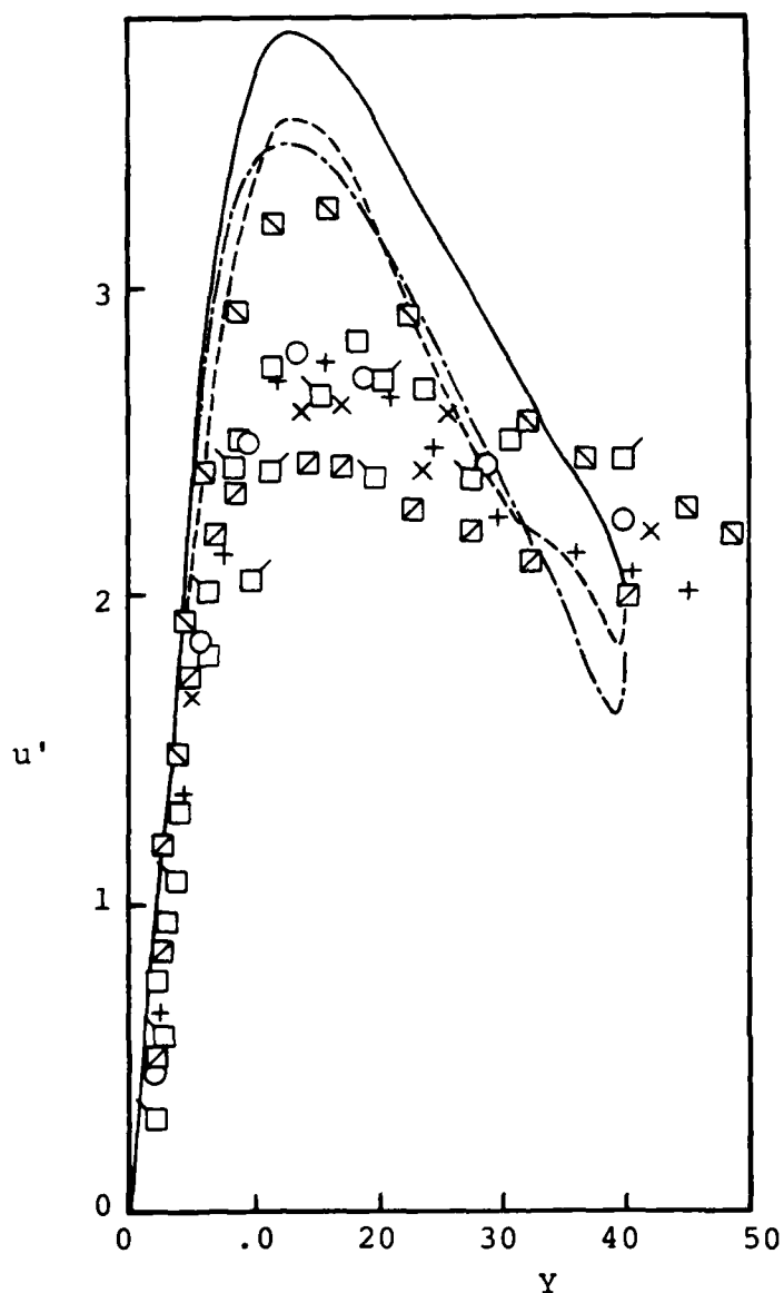
Figure 5. Intensity of velocity fluctuations.
