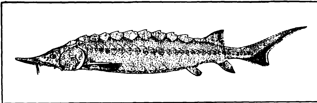
Figure 1. Atlantic sturgeon.
