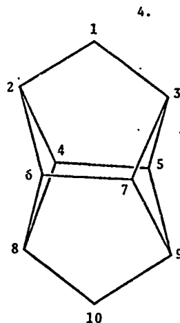
para-BISHOMOCUBANE
