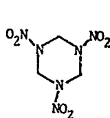
RDX
