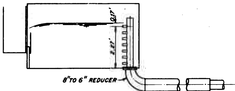
SECTION
