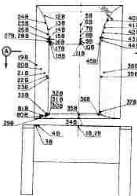
FACE VIEW
