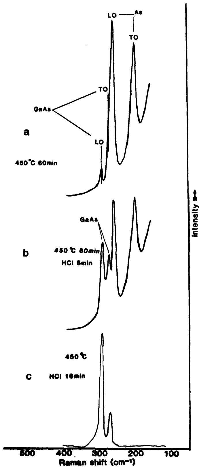
Figure 11. Raman Spectra Obtained from a Film on GaAs Generated at 450^\circ\text{C} Then Etched for 8 and 16 Minutes in a 1:1 Solution of HCl: \text{H}_2\text{O}
