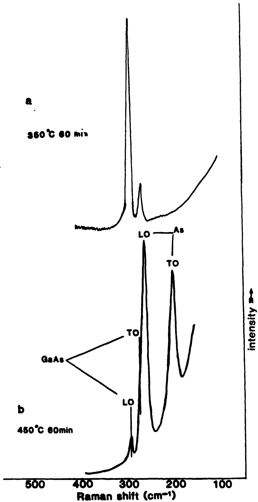
Figure 8. Raman Spectra of Thermally Treated GaAs Crystals at 350^\circ\text{C} (a), and 450^\circ\text{C} (b)
