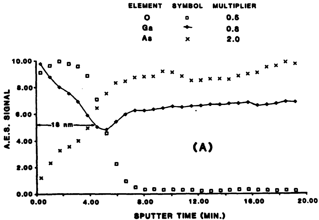
Figure 13. Auger Sputter Profiles of O, Ga, and As from Thermally Oxidized (450°C, 60 min.) GaAs Constructed from d(E \cdot N)/dE Peak-to-Peak Height (A) and (B) Same as A Except Ga Profile Constructed from Area Under E \cdot N Peak
