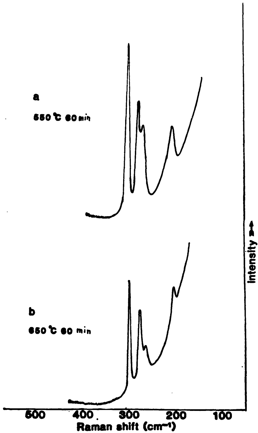
Figure 9. Raman Spectra of Thermally Treated GaAs Crystals at 550°C (a), and 650°C (b)
