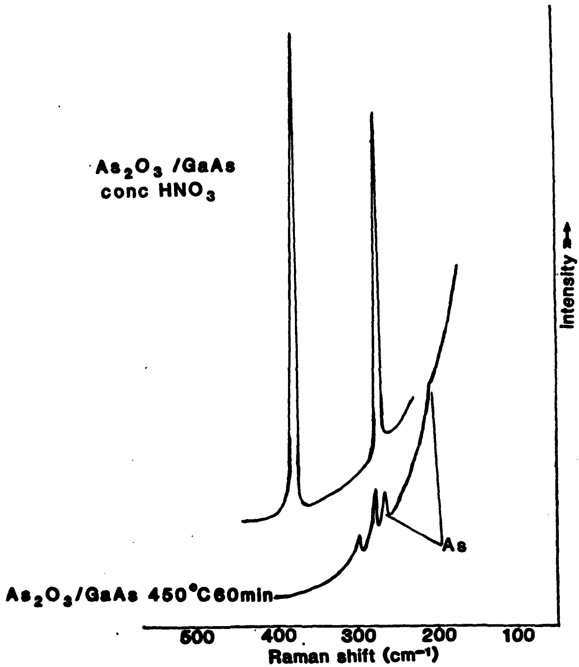
Figure 12. Raman Spectra Obtained from a Film on GaAs Generated by a 20 Second Dip in Concentrated HNO 3 Acid Then Annealed at 450°C for 60 Minutes
