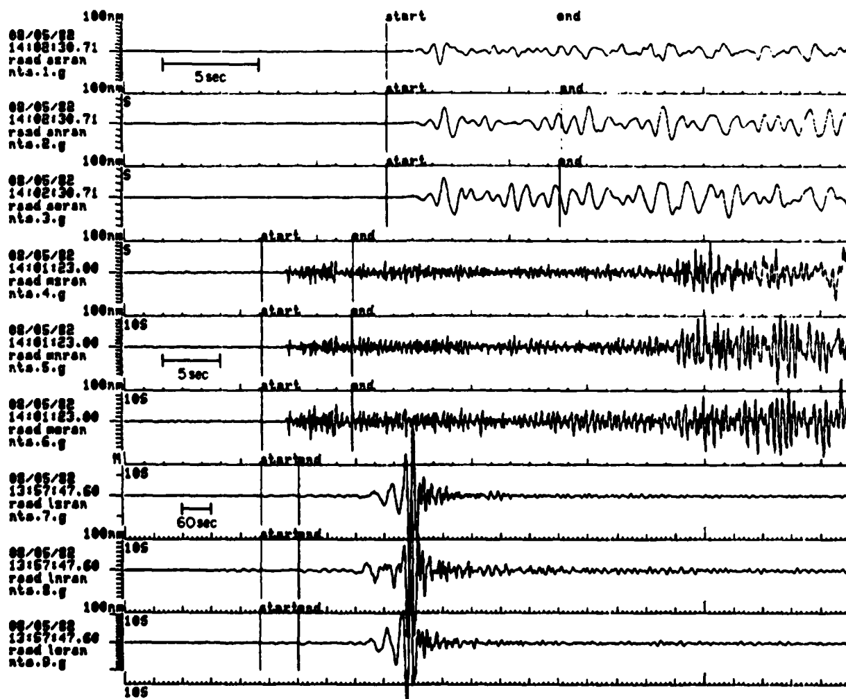
Figure 3 NTS-to-RSSD ( 11.49^{\circ} ) from top to bottom: Short period Z,N,E (40 seconds) Mid period Z,N,E (375 seconds) and Long period Z,N,E (1500 seconds) The vertical scale tick marks are 100nm for each trace, except the long period Z. The tick marks for the LPZ are 1 micron increments. The P wave window for spectral estimation in Figure 4 is shown on each seismogram indicated by the vertical bars labeled "start" and "end". Noise windows were selected prior to the P arrival. The P character of P is clear on the short period Z with strong n radial polarization. Lg is clearly observable on the Mid period band and L R is well recorded on the long period band. The P wave is not detectable on the long period.
