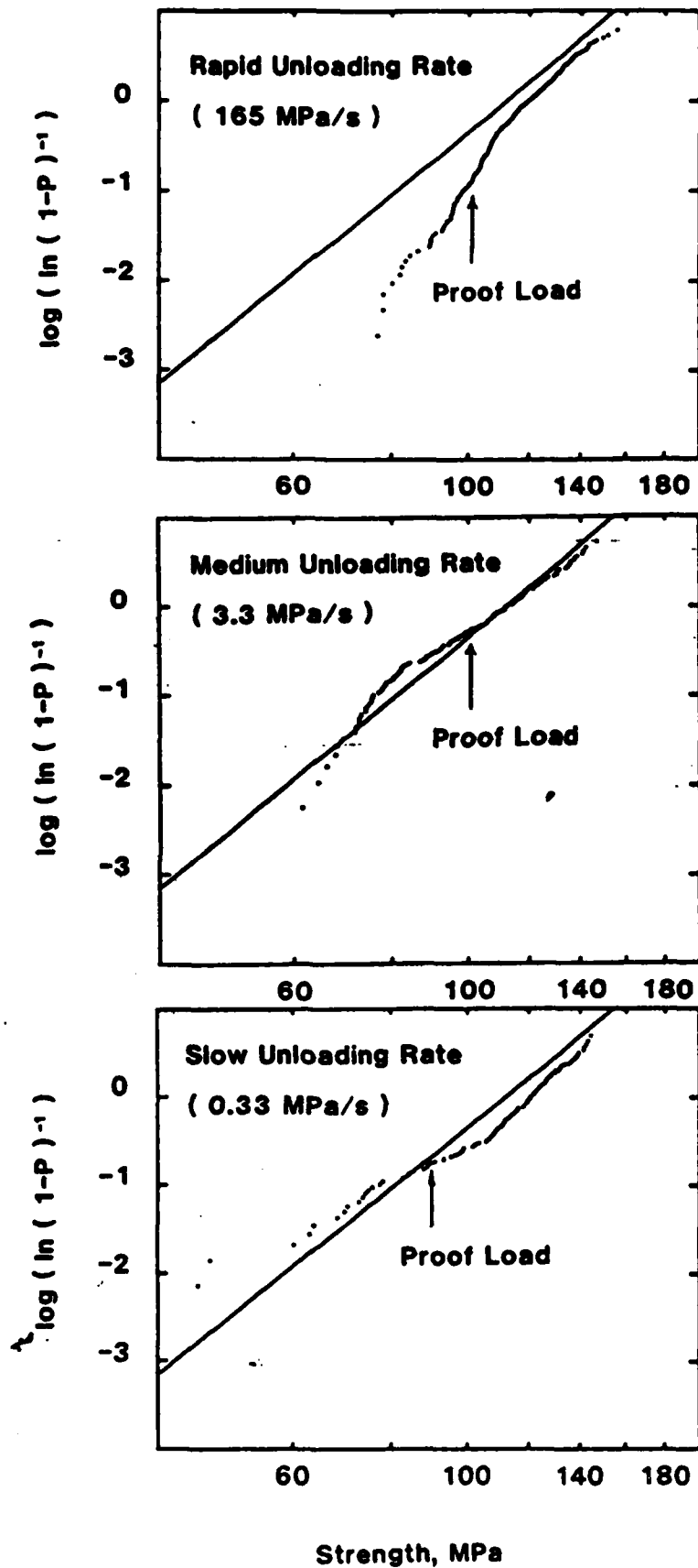
3. Strength distribution after proof testing in heptane: (a) rapid (165 MPa/s) unloading rate; (b) medium (3.3 MPa/s) unloading rate; (c) slow (0.33 MPa/s) unloading rate.
