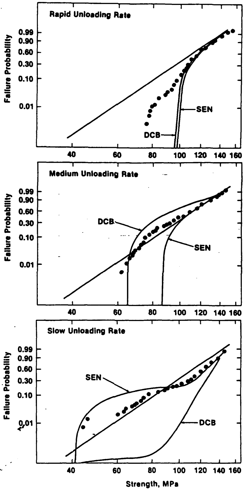
4. Strength distribution curves after proof testing in heptane, calculated from v - K_1 data shown in figure 1: (a) rapid (165 MPa/s) unloading rate; (b) medium (3.3 MPa/s) unloading rate; (c) slow (0.33 MPa/s) unloading rate.
