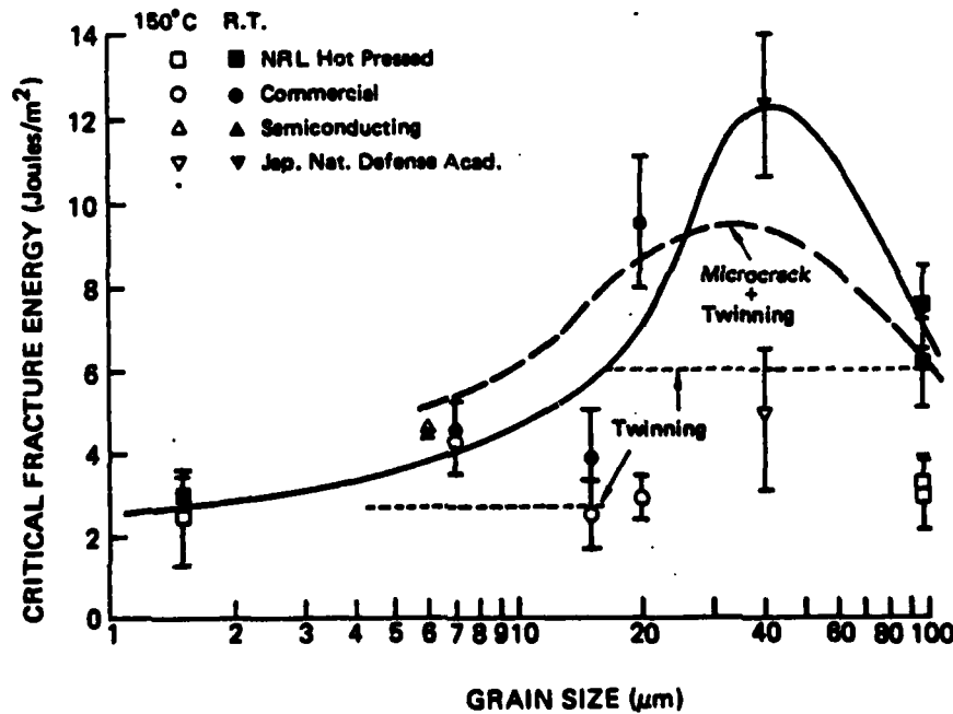
FIGURE 2 Fracture energy of \text{BaTiO}_3 as a function of grain size: best fit to room temperature data; contribution due to twinning, - - - combined effect of twinning and microcracking predicted by model of Rice and Freiman (1981).
