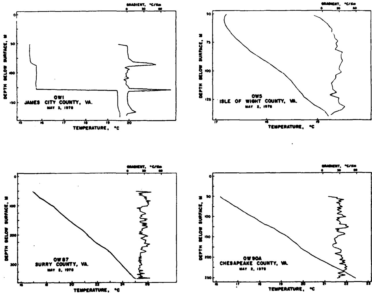
Figure 14. Temperature logs from observation wells shown in Figure 12.
