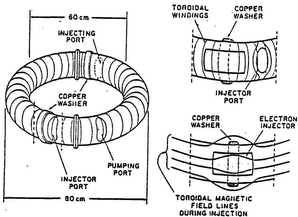
Figure 1. Betatron Experiment
