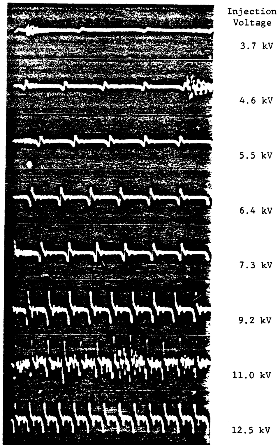
Figure 6. Oscilloscope traces of electrostatic oscillations for different injection voltages.
