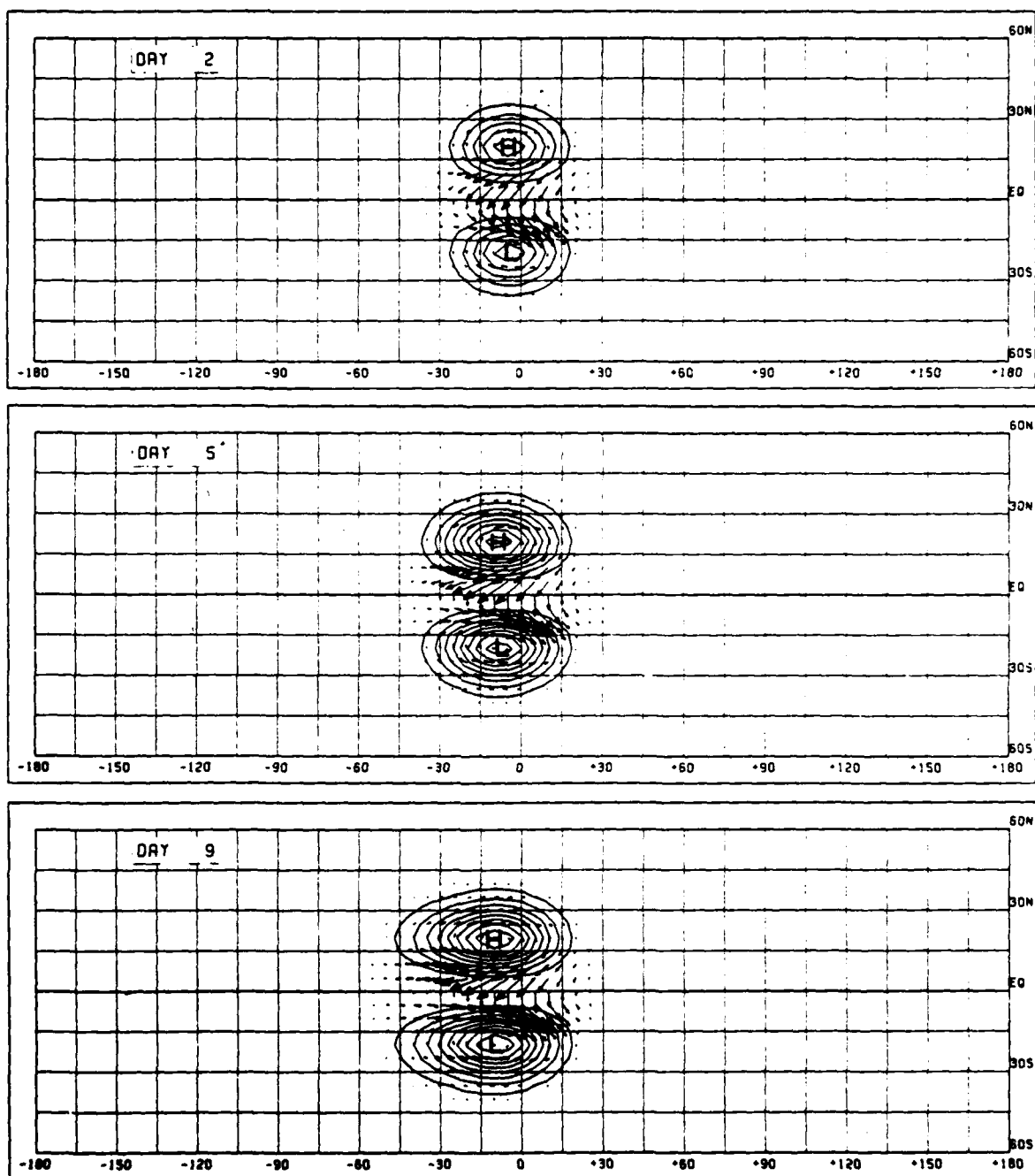
FIG. 3. Same as in Fig. 2 except for a heating function of the form Q = y \exp[-\frac{1}{4}(x^2 + y^2)]H(t) .
