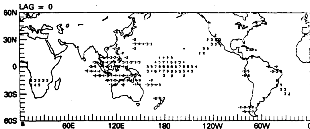
FIG. 10a. As in Fig. 5b, but with the SO signal removed.
