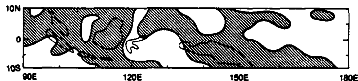
FIG. 6. Averaged signal-to-noise ratio distribution over Days 0-7. Shaded areas denote values of S \geq 1 , indicating more reliable composite values.
