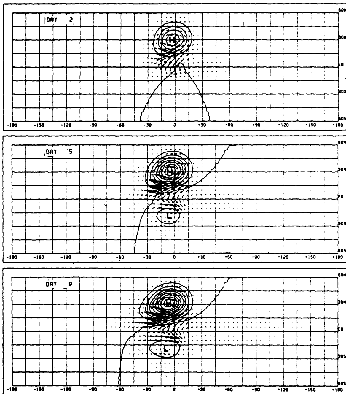
FIG. 8. Low-level wind and geopotential response for heating corresponding to a sudden turn-on of a mass source at 27^{\circ}\text{N} and an equatorial heat source of 5^{\circ}\text{S} , 36 h later with \alpha = 0.5 .
