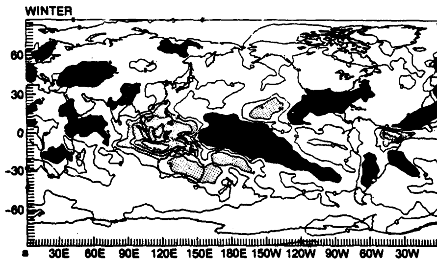
FIG. 2a. Teleconnection pattern of the difference of the composites for the dry and wet periods during winter (DW - WW as defined in the text) using the OLR variation over equatorial central Pacific as reference. Contour interval is 5 \text{ W m}^{-2} . Positive values in excess of 5 \text{ W m}^{-2} are stippled dark. Negative values less than -5 \text{ W m}^{-2} are stippled light.
