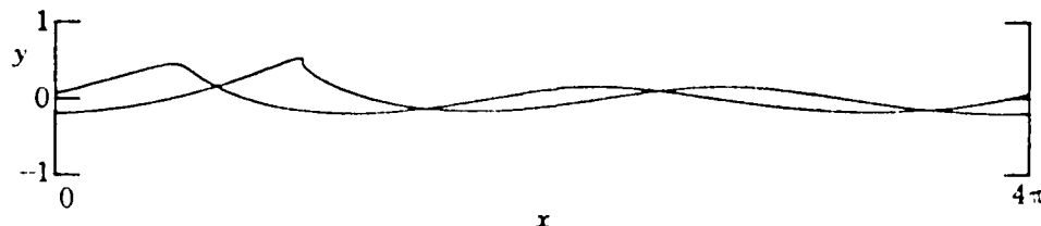
Figure 10 Profiles of an unstable mode for the overturning of a steep gravity wave with ak = 0.25 . The normalized time interval between the profiles is \Delta t = 2\pi/4 ; from Longuet-Higgins and Cokelet (1978).
