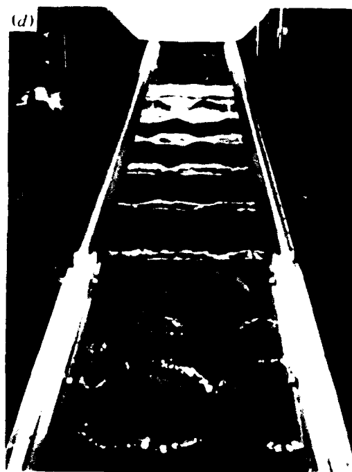
Figure 2 Spilling breakers in a laboratory wave channel; from Melville (1982). Left hand column, ak = 0.315 ; right hand, ak = 0.321 .
