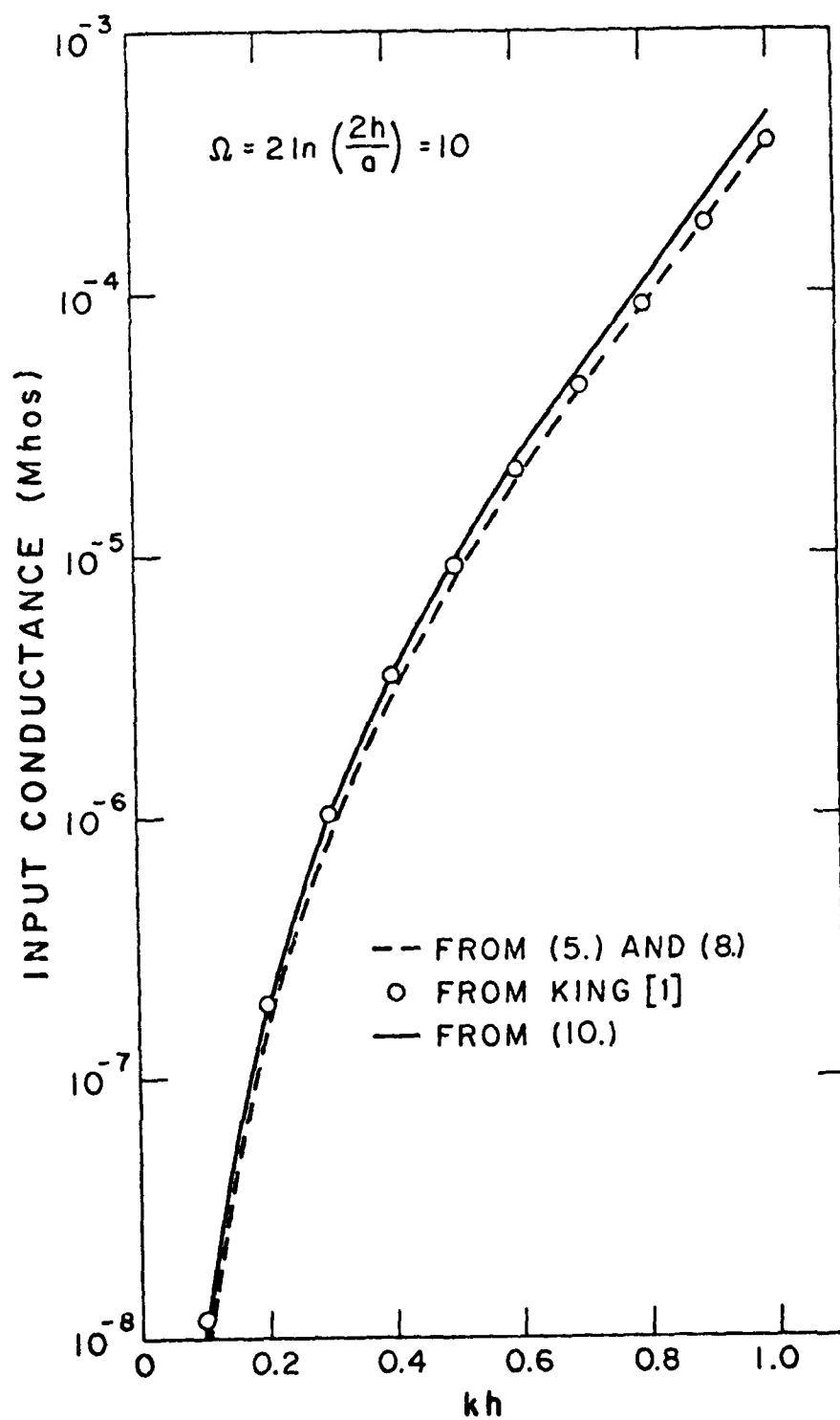
Figure 3. Input conductance of a short cylindrical antenna.
