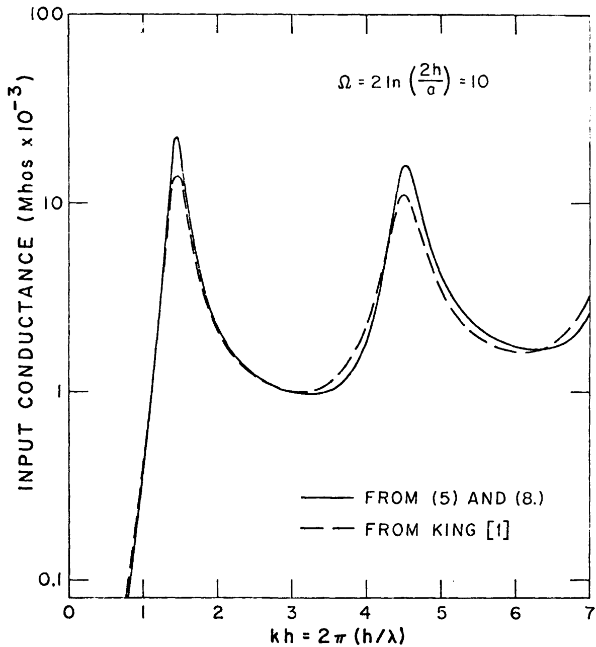
Figure 2. Input conductance of a finite length thin cylindrical antenna.
