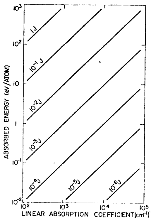
Fig. 20.9 Energy absorbed per atom by a target 10 cm from an X-ray laser, as a function of the linear absorption coefficient, for the given energy outputs by a hypothetical X-ray laser having a 10^{-3} rad divergence. A nominal interatomic spacing of 2.5 Å was assumed in order to obtain this universal plot.
