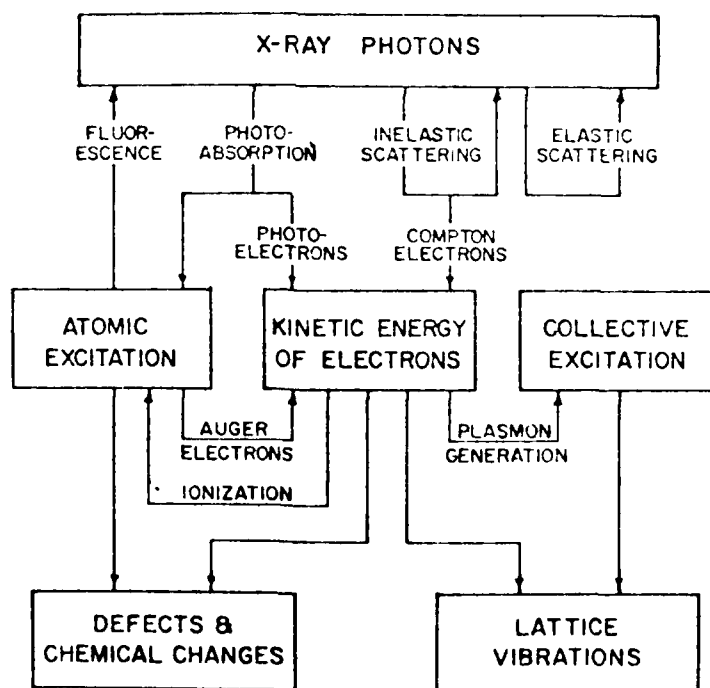
Fig. 20.13 Flow diagram for the photophysical processes by which X-ray photon energy is converted first to electronic vibrations and then to defects, chemical changes and lattice vibrations (heat) 75 .
