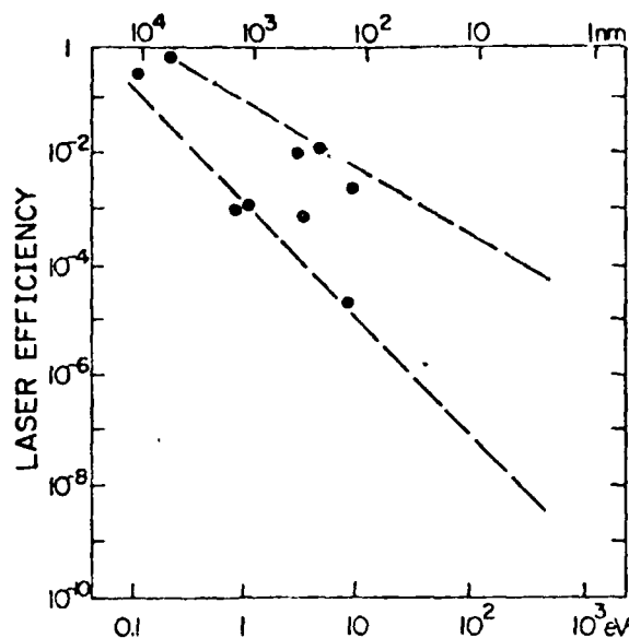
Fig. 20.7 Measured laser efficiencies as a function of laser photon energy plotted by Rhodes and Hoff 20 . The dashed lines indicate a wide region of projected efficiencies for higher-energy lasers.
