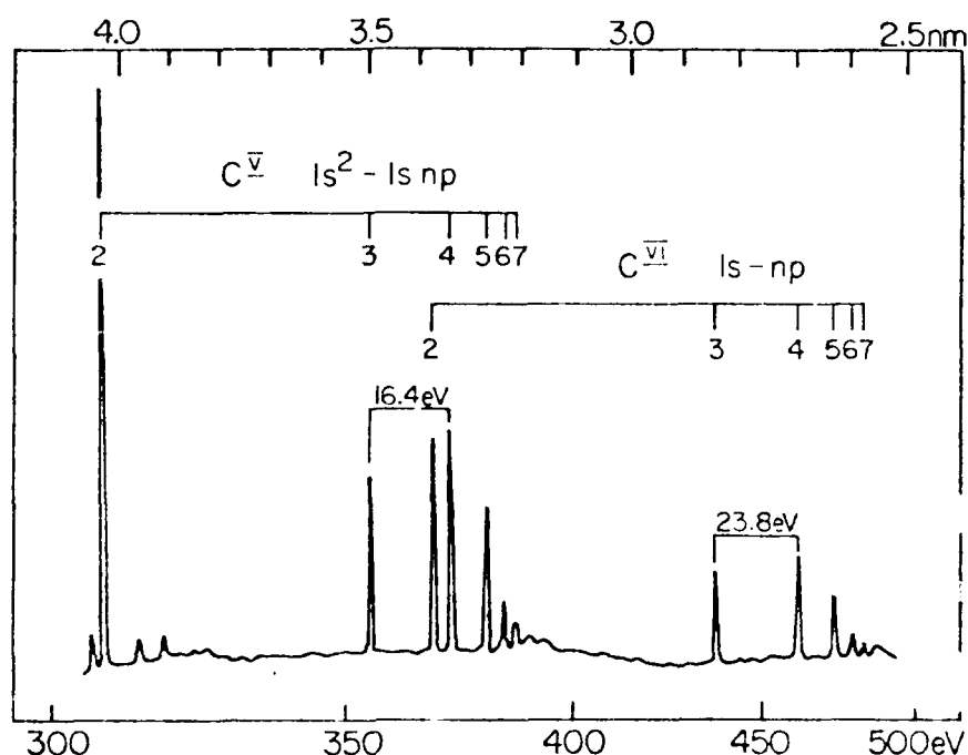
Fig. 20.6 Densitometer trace of the spectrum obtained 16 ns from a laser-heated carbon target with background gas of a few Torr pressure by Dixon and Elton 40 . The energy separation of lines from inverted levels is indicated.
