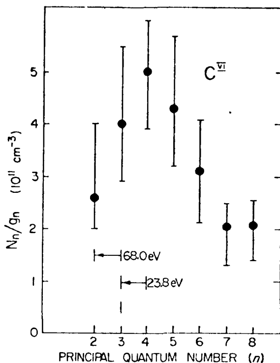
Fig. 20.5 Level population densities obtained by Irons and Peacock 38 from space-resolved spectra 2.8 mm from a laser-heated carbon target. Photon energies between inverted levels are indicated.
