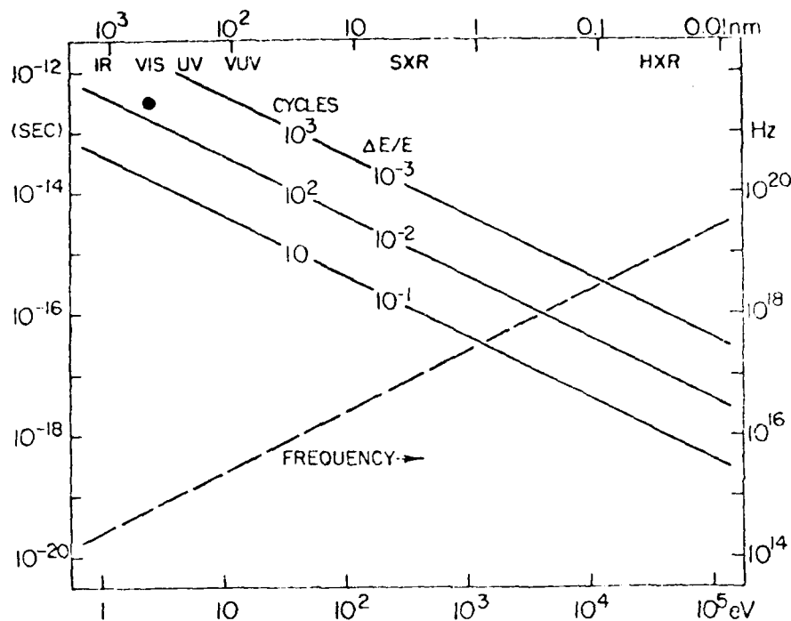
Fig. 20.8 Plot of laser pulse length vs. laser photon energy as a function of the number of cycles in the laser pulse and the relative line width \Delta E/E from the Uncertainty Principle. The dot indicates the sub-ps pulse length already demonstrated with a Nd laser 50 . The relationship between electromagnetic frequency and photon energy is also given (dashed line).
