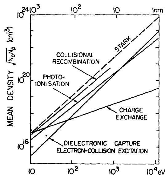
Fig. 20.4 Mean density of ground-state ( N_0 ) and pump ( N_p ) particles necessary for laser action with a gain coefficient of five calculated as a function of laser output photon energy for various mechanisms by Elton and his colleagues 6,22 . Stark broadening sets a limit (dashed line) on useful densities.
