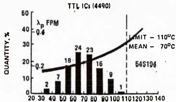
SAMPLE IC FAILURE RATES vs JUNCTION TEMPERATURE
