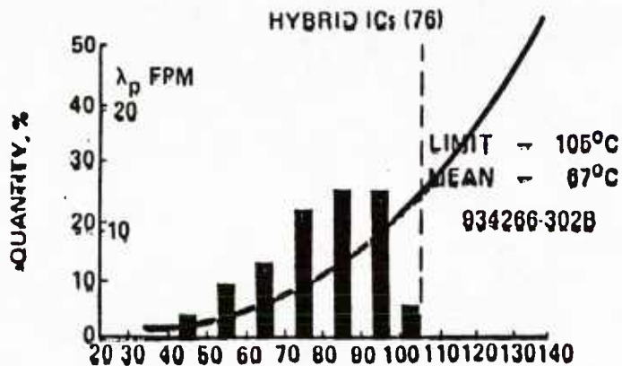
SAMPLE IC FAILURE RATES vs JUNCTION TEMPERATURE
