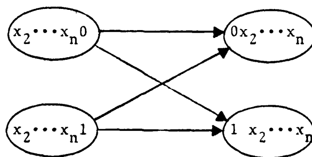
Fig. 2.3 Adjacency Quadruple.
