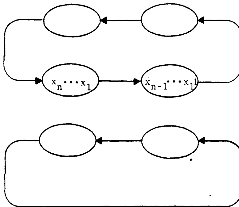
Fig. 4.5 Two Cycle Graph.
