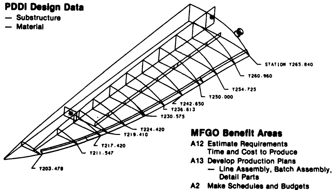
Figure 16. - Conceptual analysis - substructure definition.
