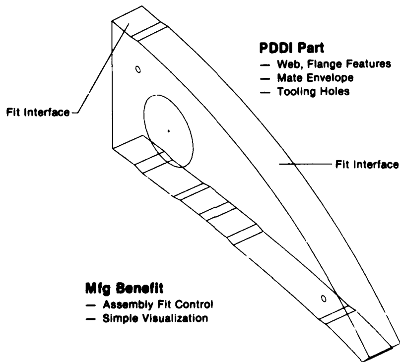
Figure 20. - Detailed analysis - part interface.
