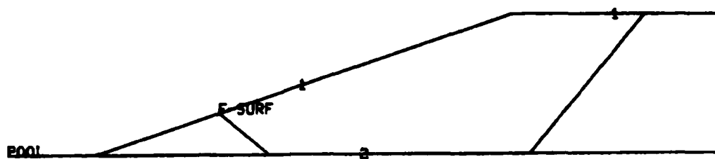
Figure 20. Display of failure surface from wedge analysis
