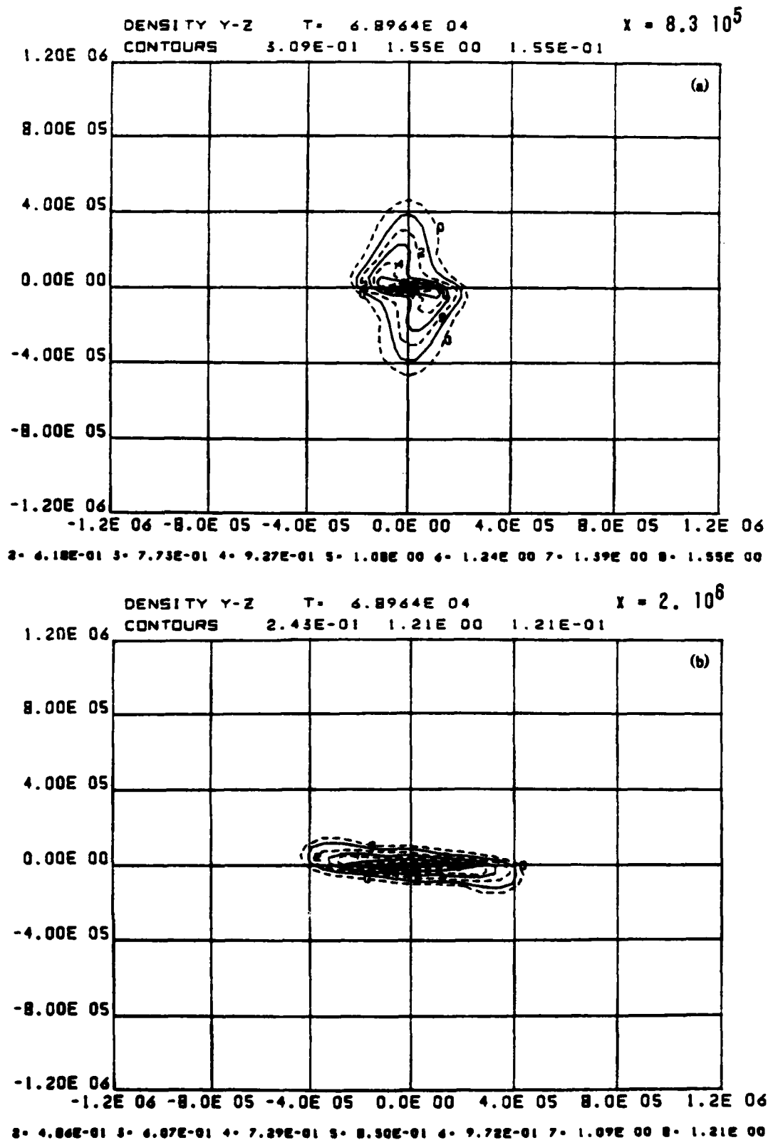
Fig. 6. Plasma density contours in cross-sectional planes perpendicular to the solar wind 6 hours after the 90° rotational discontinuity. Figure (a) shows a cross-sectional plane 8.3 \times 10^5 km behind the comet nucleus and (b) shows a cross-sectional 2 \times 10^6 km behind. Note the twisting of the plasma sheet from outside inward.
