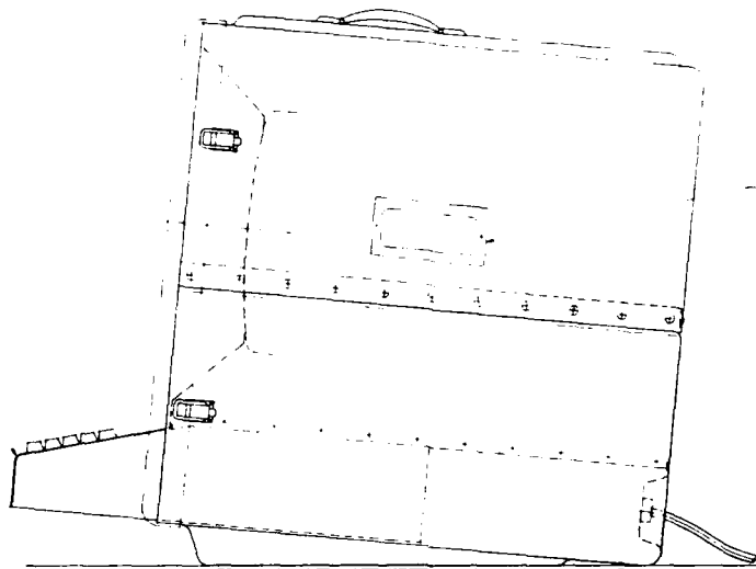
SIDE VIEW - TERMINAL CONTAINER KEYBOARD TRAY EXTENDED - COVER REMOVED
