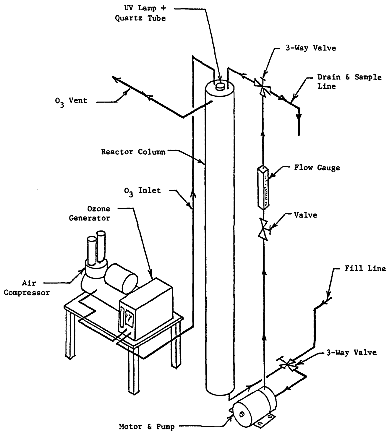
Figure 7. Reactor Schematic.
