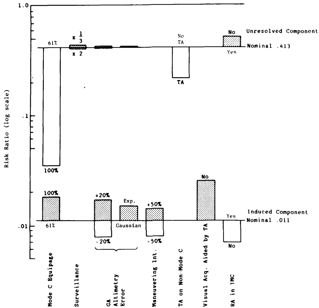
FIGURE 5 INFLUENCE OF VARIOUS FACTORS ON OVERALL SYSTEM PERFORMANCE
